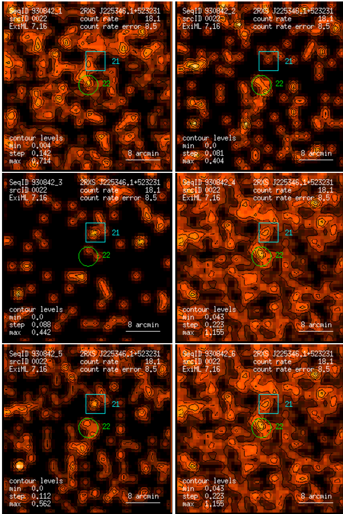
Figure 22: RASS 930842: detection 0022: band rate images, Gaussian filter: (1) PSPC channels 11 – 41, (2) 52 – 90, (3) 91 – 201, (4) 11 – 235, (5) 52 – 201, (6) 11 – 201. Broad band rates in counts/ks. Band rate contour levels in counts/ks/arcmin 2 .
