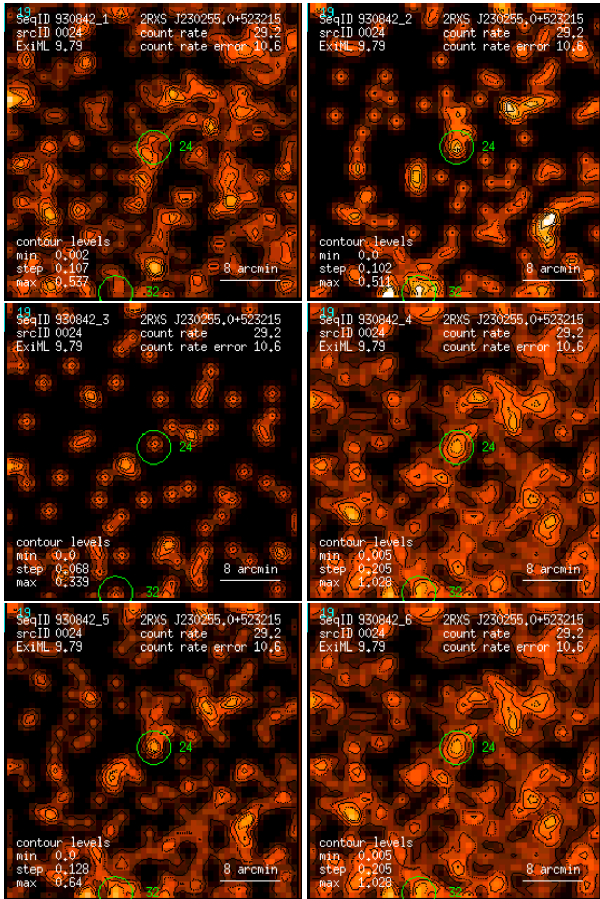
Figure 24: RASS 930842: detection 0024: band rate images, Gaussian filter: (1) PSPC channels 11 – 41, (2) 52 – 90, (3) 91 – 201, (4) 11 – 235, (5) 52 – 201, (6) 11 – 201. Broad band rates in counts/ks. Band rate contour levels in counts/ks/arcmin 2 .
