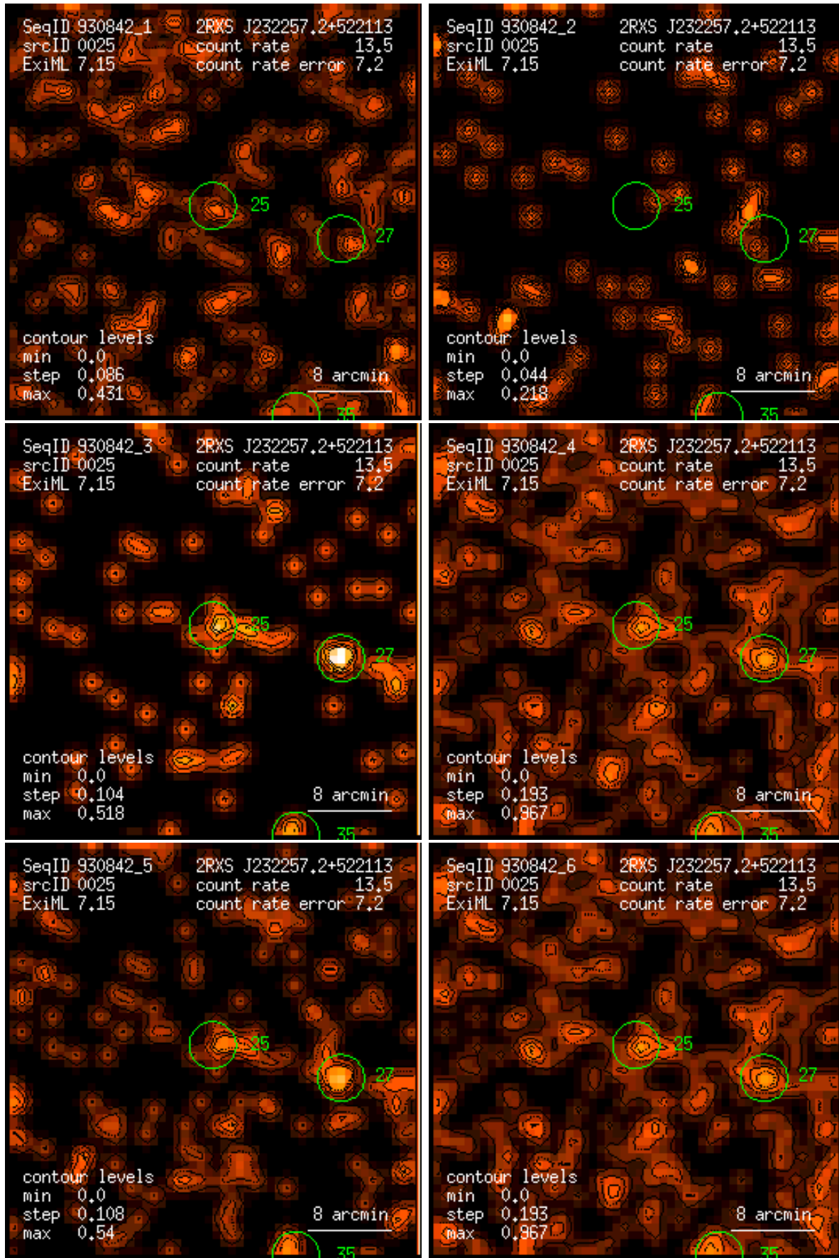
Figure 25: RASS 930842: detection 0025: band rate images, Gaussian filter: (1) PSPC channels 11 – 41, (2) 52 – 90, (3) 91 – 201, (4) 11 – 235, (5) 52 – 201, (6) 11 – 201. Broad band rates in counts/ks. Band rate contour levels in counts/ks/arcmin 2 .
