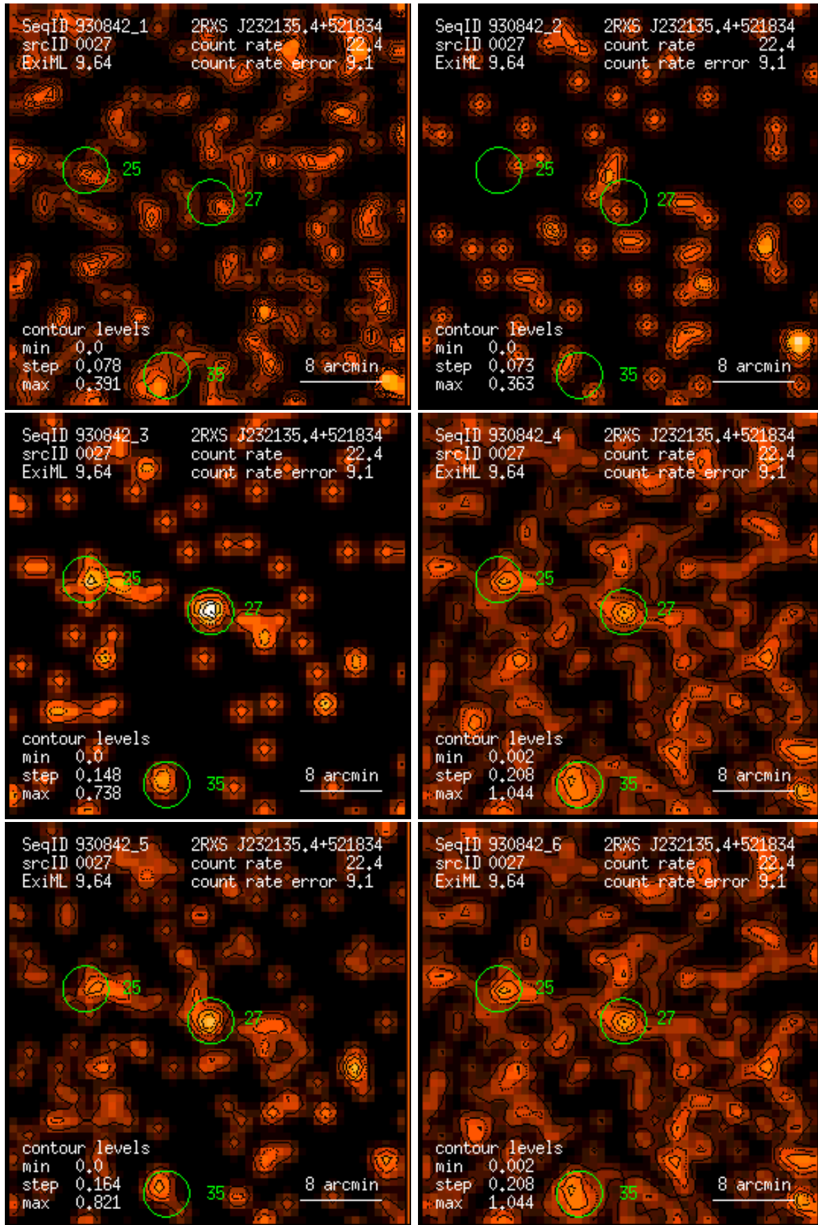
Figure 27: RASS 930842: detection 0027: band rate images, Gaussian filter: (1) PSPC channels 11 – 41, (2) 52 – 90, (3) 91 – 201, (4) 11 – 235, (5) 52 – 201, (6) 11 – 201. Broad band rates in counts/ks. Band rate contour levels in counts/ks/arcmin 2 .
