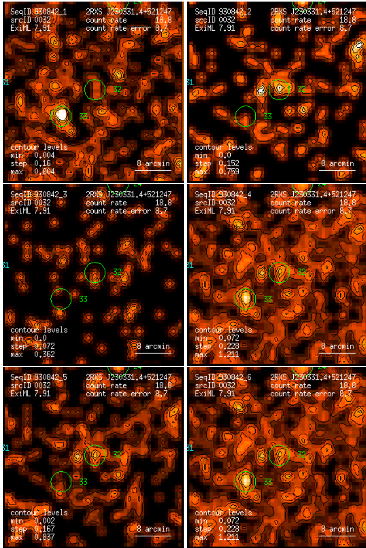
Figure 32: RASS 930842: detection 0032: band rate images, Gaussian filter: (1) PSPC channels 11 – 41, (2) 52 – 90, (3) 91 – 201, (4) 11 – 235, (5) 52 – 201, (6) 11 – 201. Broad band rates in counts/ks. Band rate contour levels in counts/ks/arcmin 2 .
