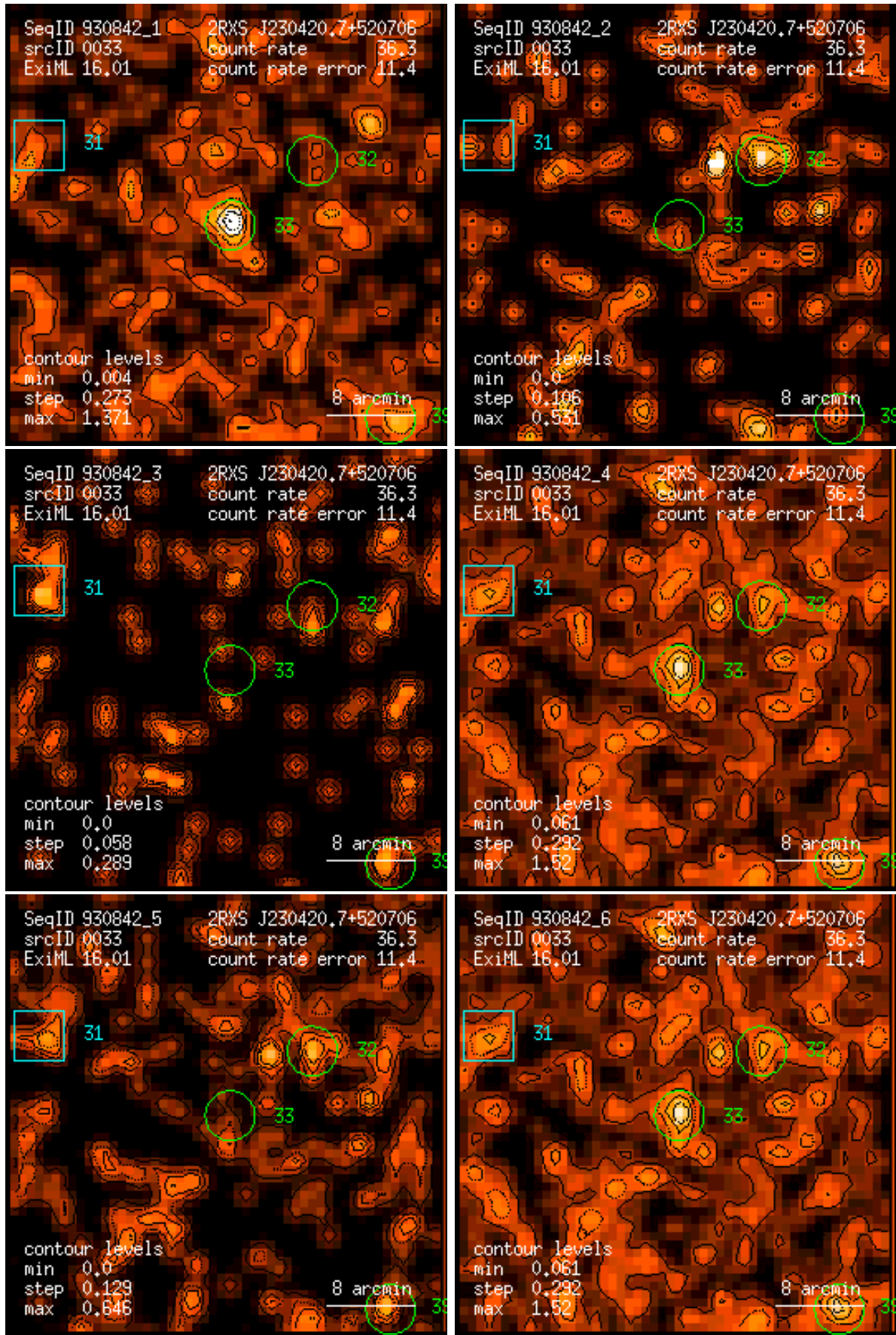
Figure 33: RASS 930842: detection 0033: band rate images, Gaussian filter: (1) PSPC channels 11 – 41, (2) 52 – 90, (3) 91 – 201, (4) 11 – 235, (5) 52 – 201, (6) 11 – 201. Broad band rates in counts/ks. Band rate contour levels in counts/ks/arcmin 2 .
