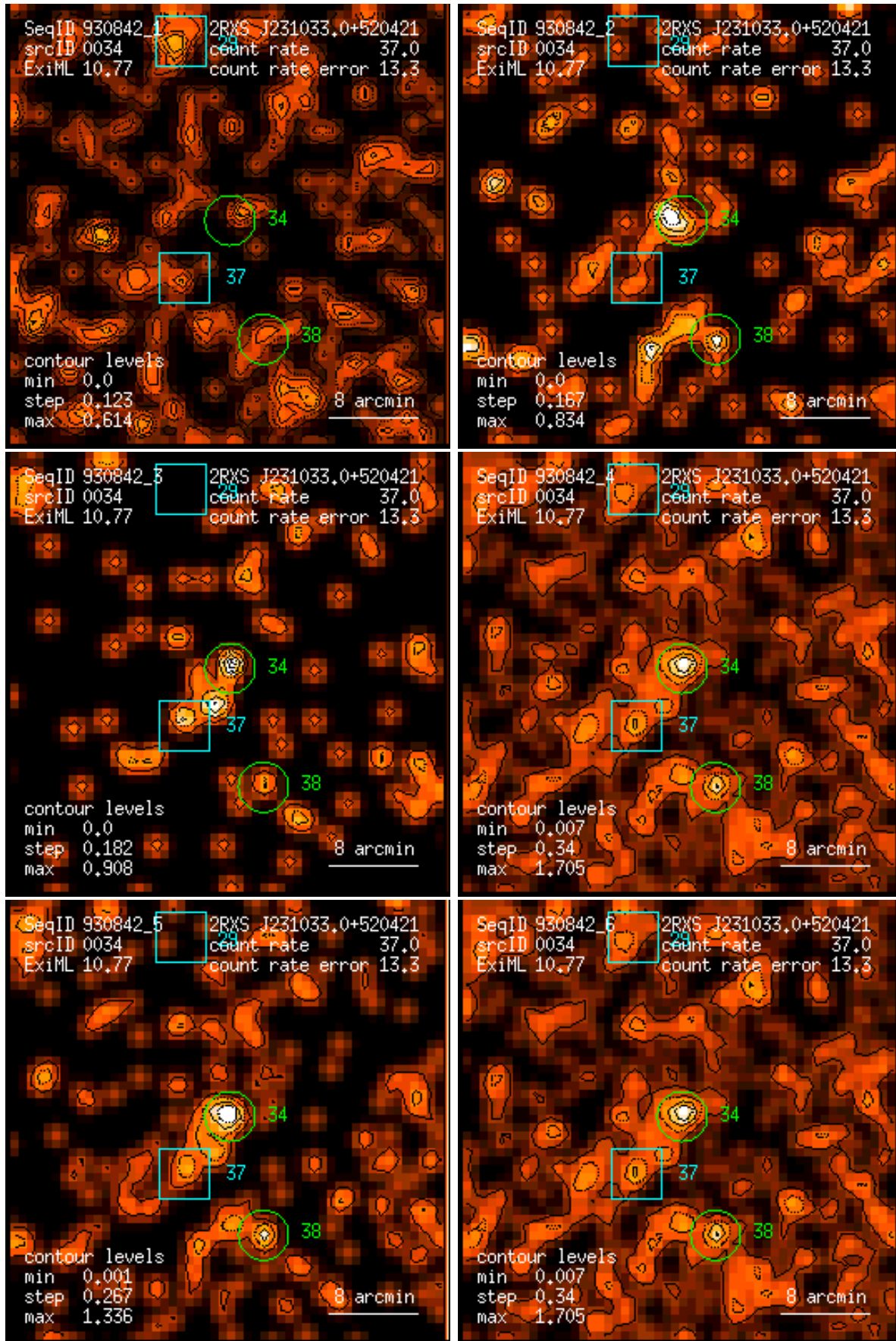
Figure 34: RASS 930842: detection 0034: band rate images, Gaussian filter: (1) PSPC channels 11 – 41, (2) 52 – 90, (3) 91 – 201, (4) 11 – 235, (5) 52 – 201, (6) 11 – 201. Broad band rates in counts/ks. Band rate contour levels in counts/ks/arcmin 2 .
