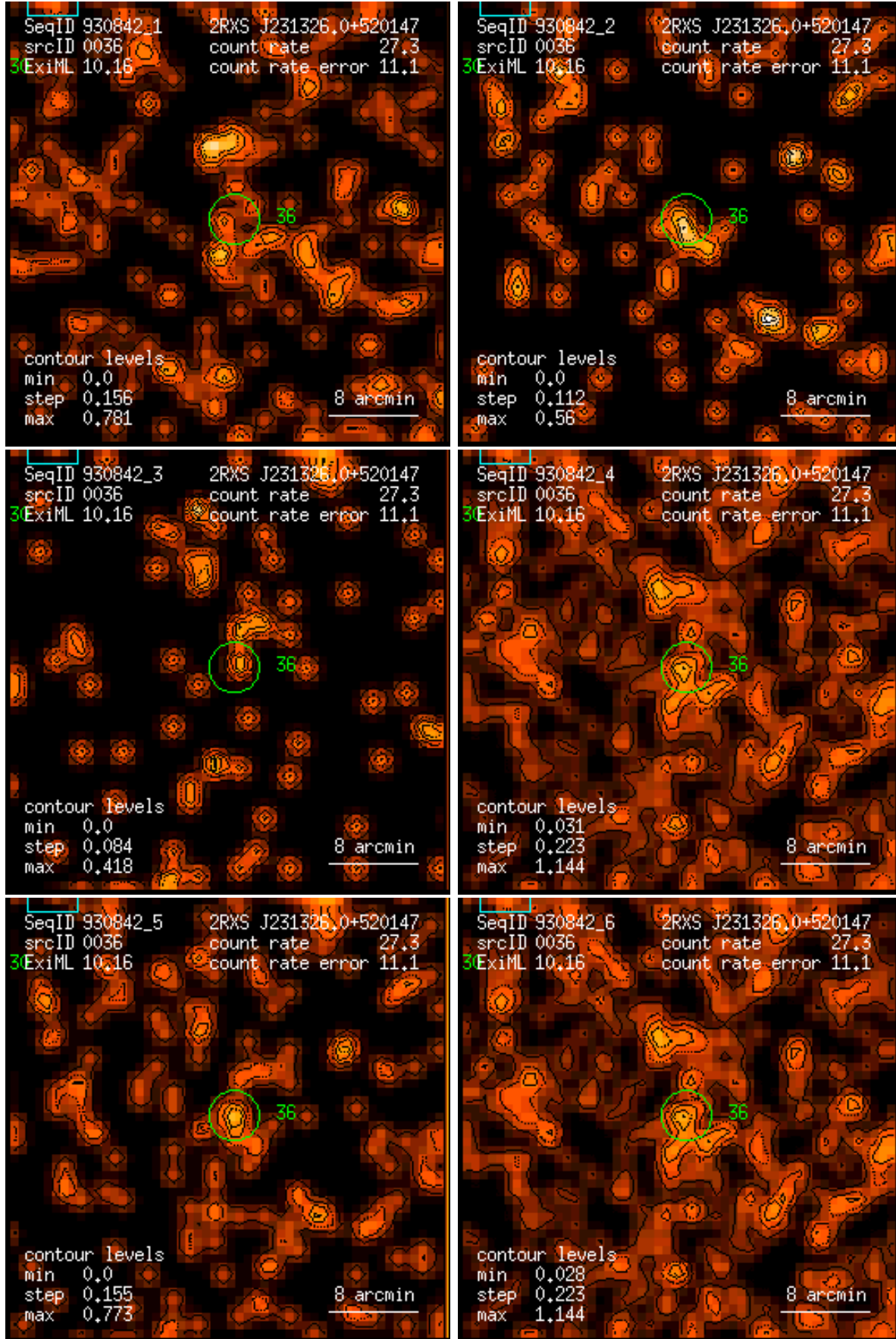
Figure 36: RASS 930842: detection 0036: band rate images, Gaussian filter: (1) PSPC channels 11 – 41, (2) 52 – 90, (3) 91 – 201, (4) 11 – 235, (5) 52 – 201, (6) 11 – 201. Broad band rates in counts/ks. Band rate contour levels in counts/ks/arcmin 2 .
