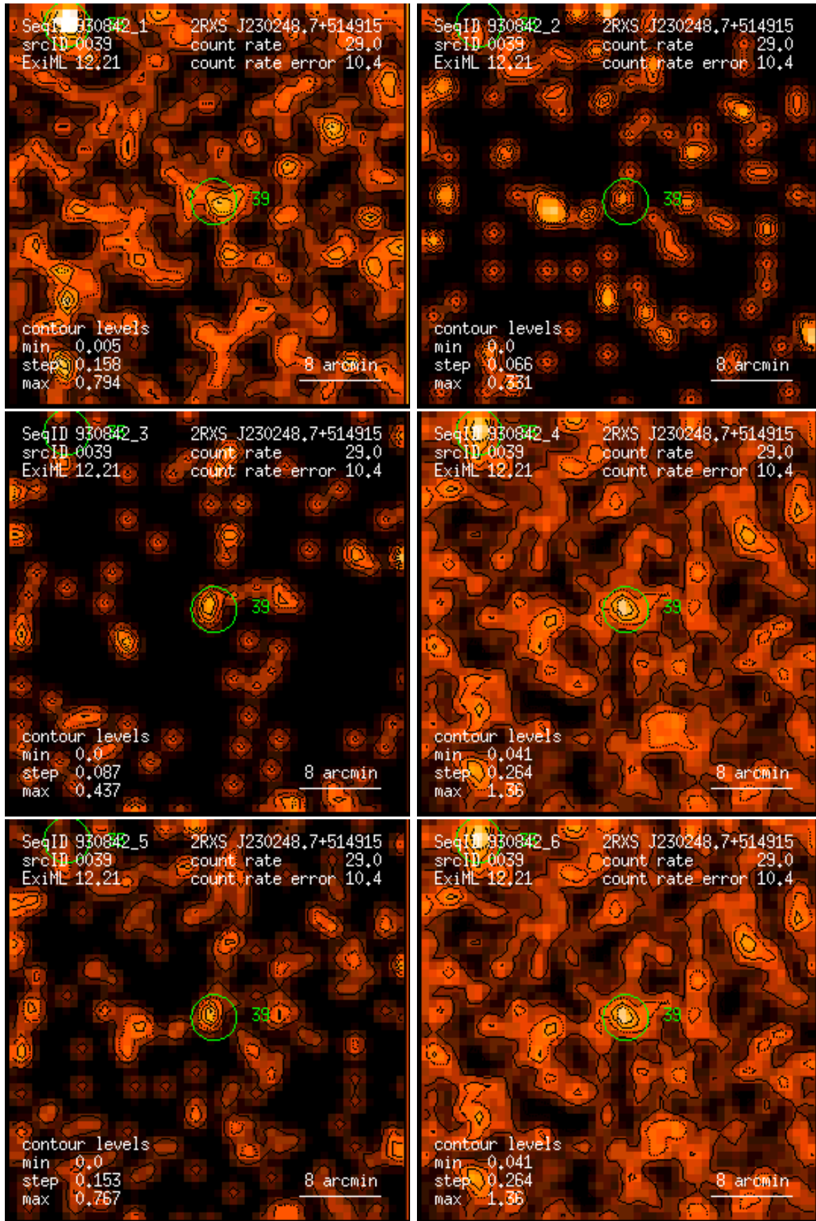
Figure 39: RASS 930842: detection 0039: band rate images, Gaussian filter: (1) PSPC channels 11 – 41, (2) 52 – 90, (3) 91 – 201, (4) 11 – 235, (5) 52 – 201, (6) 11 – 201. Broad band rates in counts/ks. Band rate contour levels in counts/ks/arcmin 2 .
