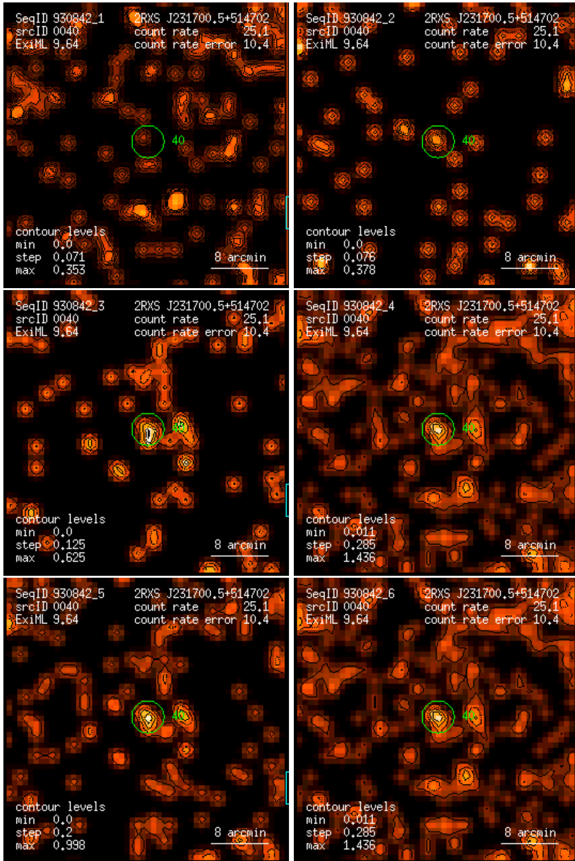
Figure 40: RASS 930842: detection 0040: band rate images, Gaussian filter: (1) PSPC channels 11 – 41, (2) 52 – 90, (3) 91 – 201, (4) 11 – 235, (5) 52 – 201, (6) 11 – 201. Broad band rates in counts/ks. Band rate contour levels in counts/ks/arcmin 2 .
