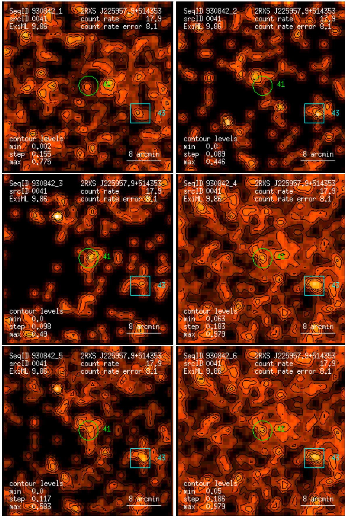
Figure 41: RASS 930842: detection 0041: band rate images, Gaussian filter: (1) PSPC channels 11 – 41, (2) 52 – 90, (3) 91 – 201, (4) 11 – 235, (5) 52 – 201, (6) 11 – 201. Broad band rates in counts/ks. Band rate contour levels in counts/ks/arcmin 2 .
