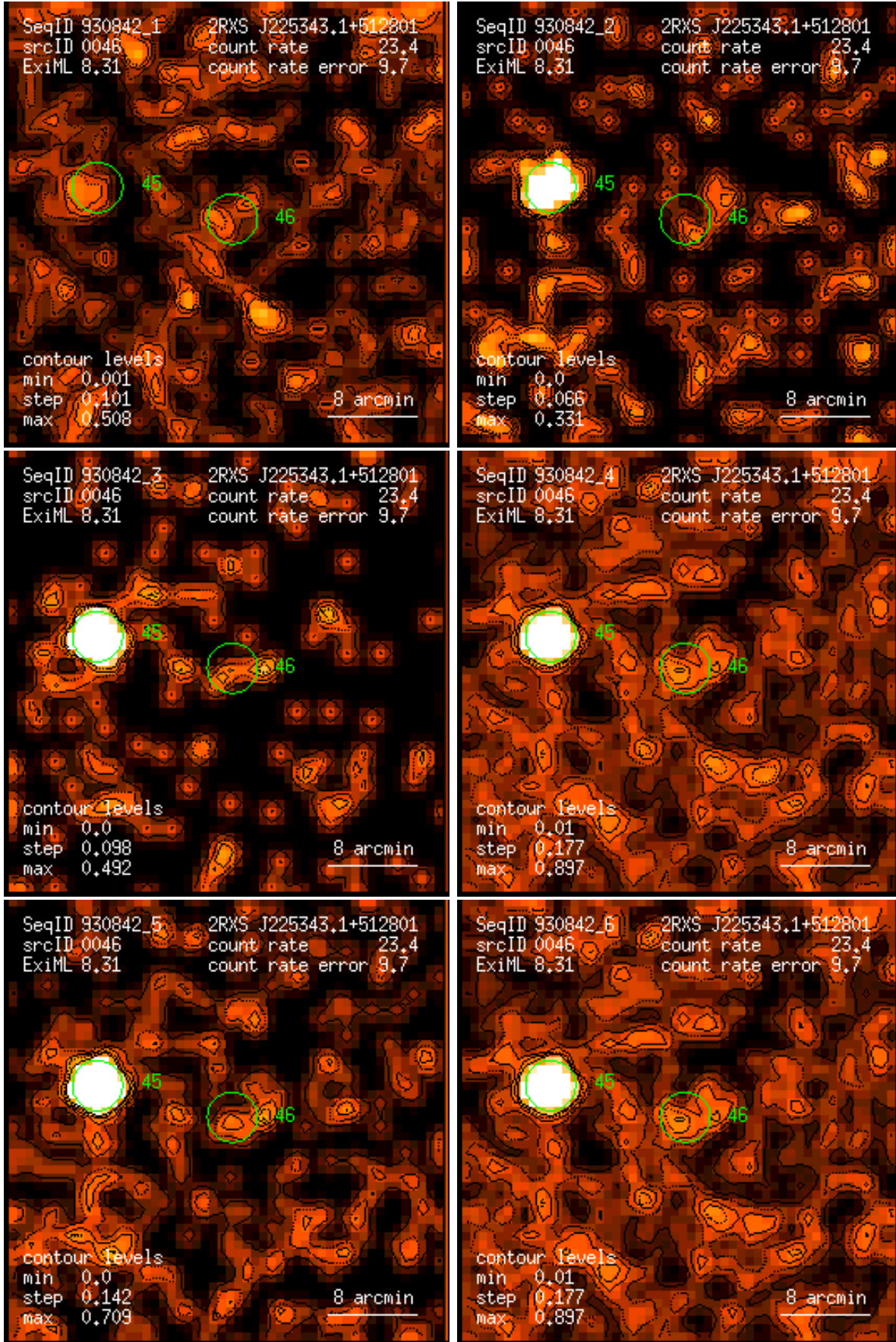
Figure 46: RASS 930842: detection 0046: band rate images, Gaussian filter: (1) PSPC channels 11 – 41, (2) 52 – 90, (3) 91 – 201, (4) 11 – 235, (5) 52 – 201, (6) 11 – 201. Broad band rates in counts/ks. Band rate contour levels in counts/ks/arcmin 2 .
