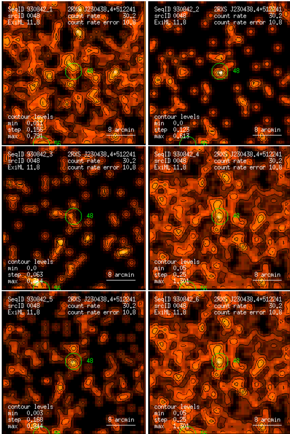
Figure 48: RASS 930842: detection 0048: band rate images, Gaussian filter: (1) PSPC channels 11 – 41, (2) 52 – 90, (3) 91 – 201, (4) 11 – 235, (5) 52 – 201, (6) 11 – 201. Broad band rates in counts/ks. Band rate contour levels in counts/ks/arcmin 2 .
