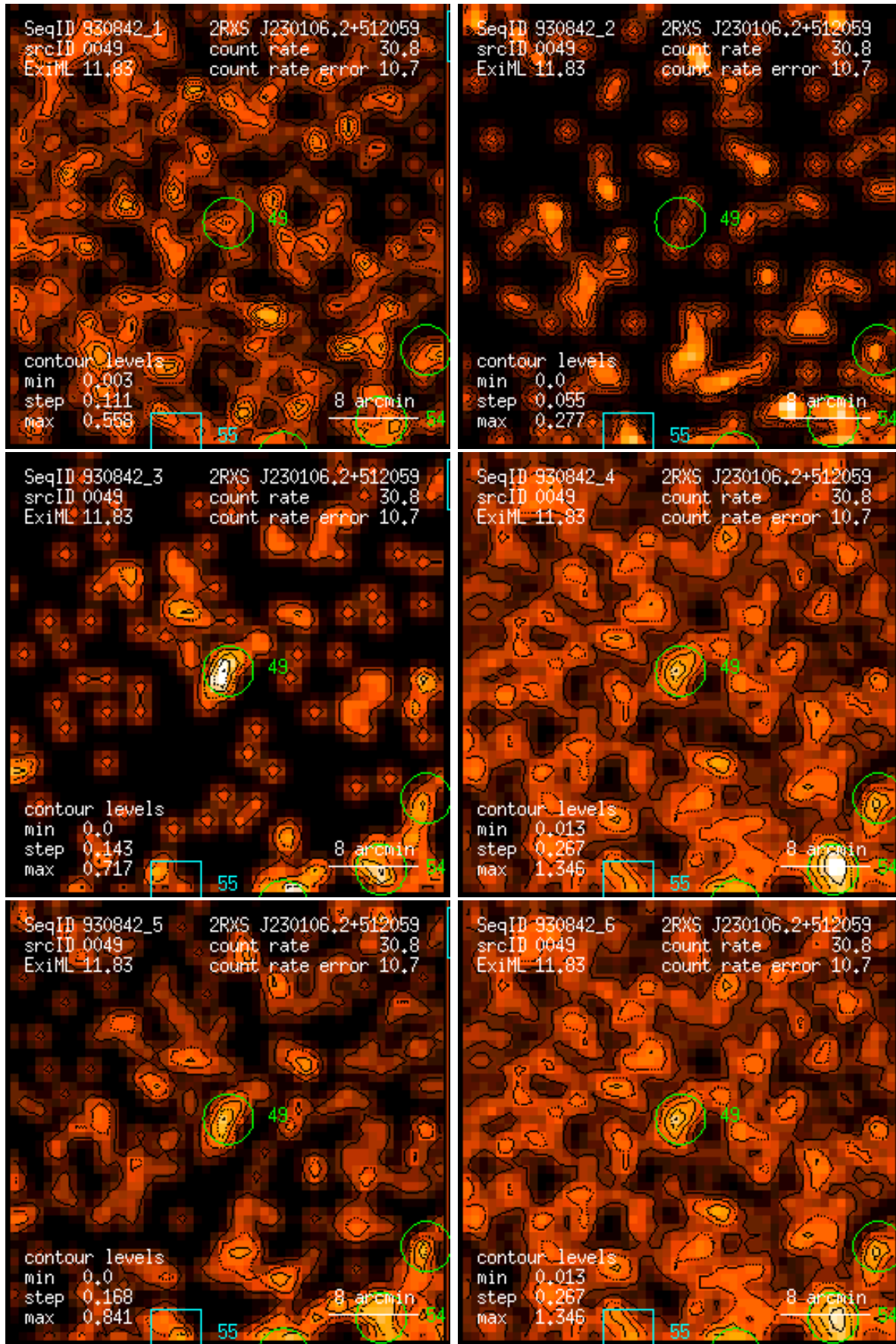
Figure 49: RASS 930842: detection 0049: band rate images, Gaussian filter: (1) PSPC channels 11 – 41, (2) 52 – 90, (3) 91 – 201, (4) 11 – 235, (5) 52 – 201, (6) 11 – 201. Broad band rates in counts/ks. Band rate contour levels in counts/ks/arcmin 2 .
