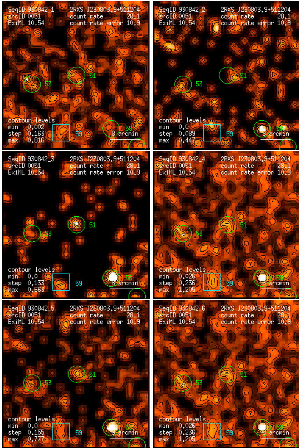
Figure 51: RASS 930842: detection 0051: band rate images, Gaussian filter: (1) PSPC channels 11 – 41, (2) 52 – 90, (3) 91 – 201, (4) 11 – 235, (5) 52 – 201, (6) 11 – 201. Broad band rates in counts/ks. Band rate contour levels in counts/ks/arcmin 2 .
