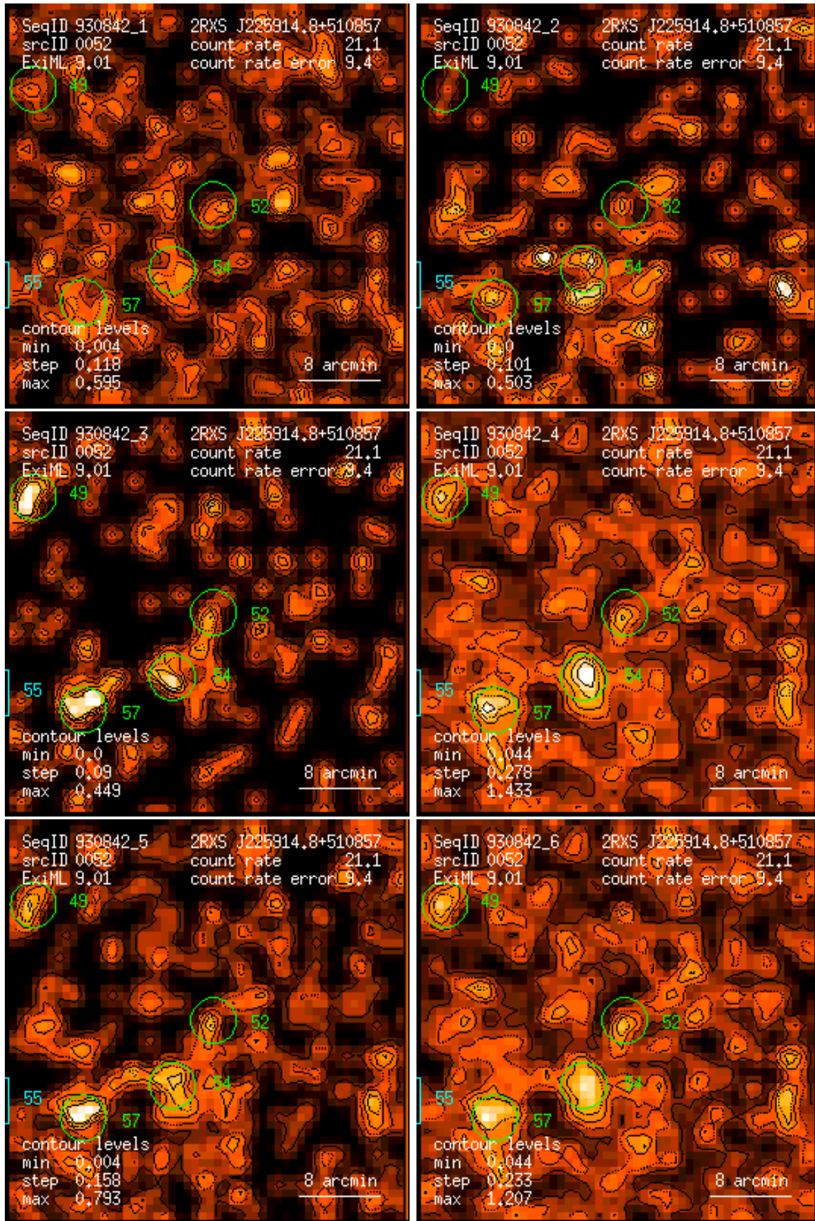
Figure 52: RASS 930842: detection 0052: band rate images, Gaussian filter: (1) PSPC channels 11 – 41, (2) 52 – 90, (3) 91 – 201, (4) 11 – 235, (5) 52 – 201, (6) 11 – 201. Broad band rates in counts/ks. Band rate contour levels in counts/ks/arcmin 2 .
