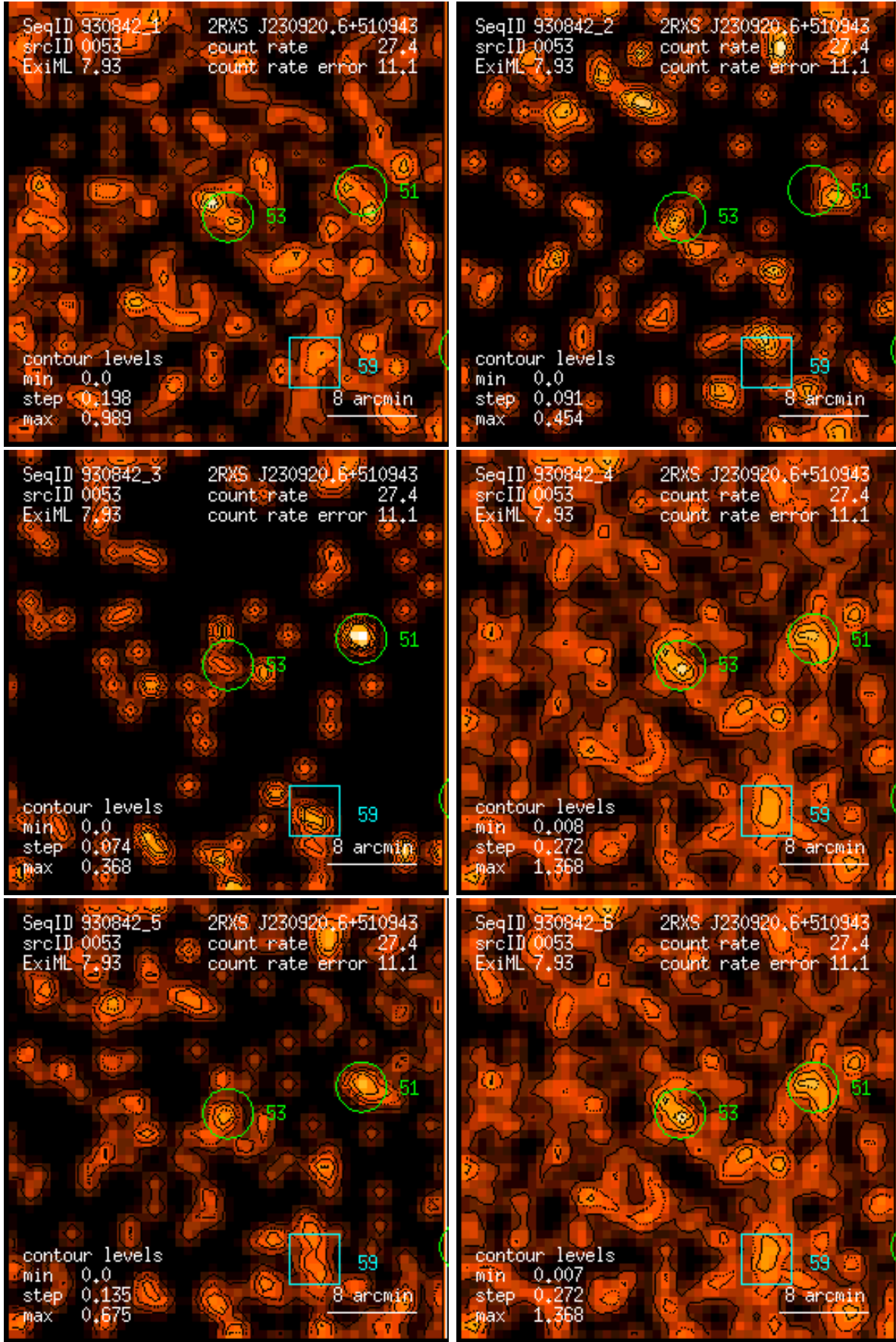
Figure 53: RASS 930842: detection 0053: band rate images, Gaussian filter: (1) PSPC channels 11 – 41, (2) 52 – 90, (3) 91 – 201, (4) 11 – 235, (5) 52 – 201, (6) 11 – 201. Broad band rates in counts/ks. Band rate contour levels in counts/ks/arcmin 2 .
