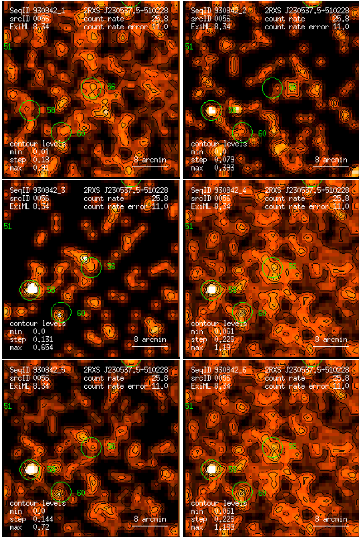
Figure 56: RASS 930842: detection 0056: band rate images, Gaussian filter: (1) PSPC channels 11 – 41, (2) 52 – 90, (3) 91 – 201, (4) 11 – 235, (5) 52 – 201, (6) 11 – 201. Broad band rates in counts/ks. Band rate contour levels in counts/ks/arcmin 2 .
