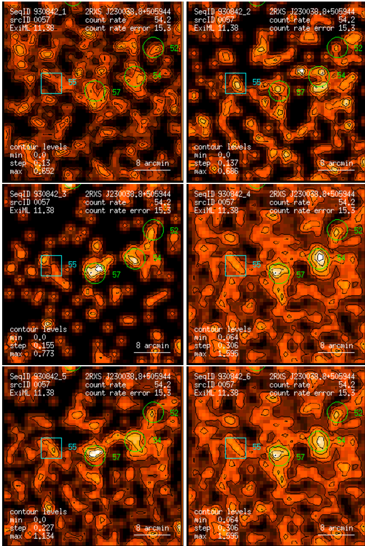
Figure 57: RASS 930842: detection 0057: band rate images, Gaussian filter: (1) PSPC channels 11 – 41, (2) 52 – 90, (3) 91 – 201, (4) 11 – 235, (5) 52 – 201, (6) 11 – 201. Broad band rates in counts/ks. Band rate contour levels in counts/ks/arcmin 2 .
