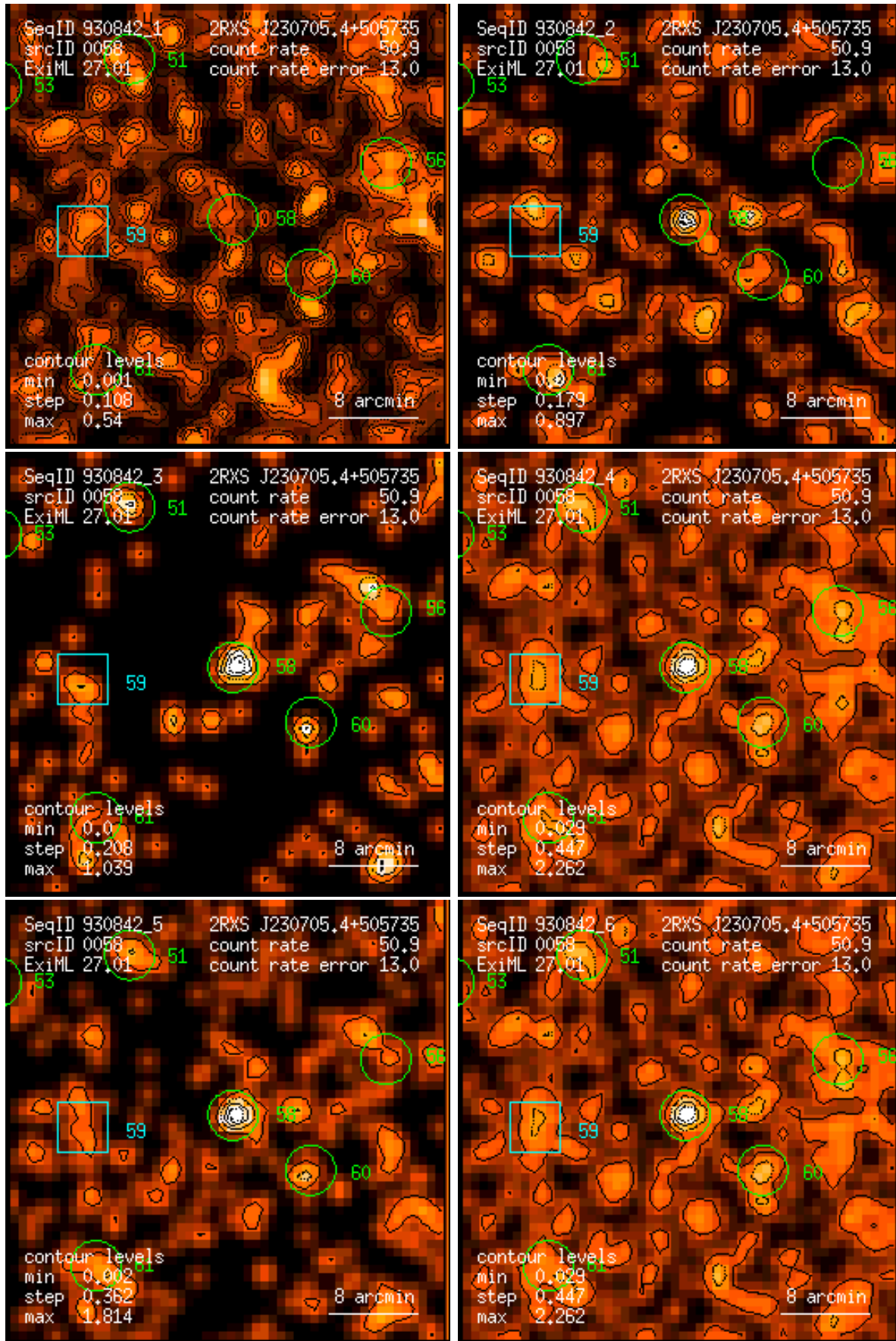
Figure 58: RASS 930842: detection 0058: band rate images, Gaussian filter: (1) PSPC channels 11 – 41, (2) 52 – 90, (3) 91 – 201, (4) 11 – 235, (5) 52 – 201, (6) 11 – 201. Broad band rates in counts/ks. Band rate contour levels in counts/ks/arcmin 2 .
