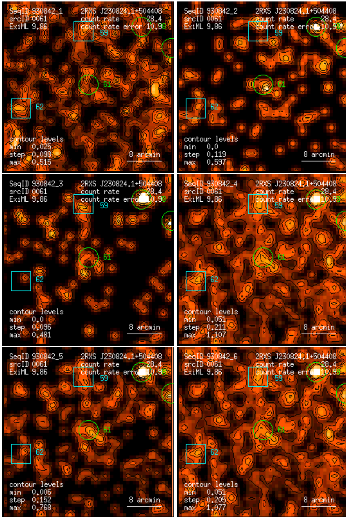
Figure 61: RASS 930842: detection 0061: band rate images, Gaussian filter: (1) PSPC channels 11 – 41, (2) 52 – 90, (3) 91 – 201, (4) 11 – 235, (5) 52 – 201, (6) 11 – 201. Broad band rates in counts/ks. Band rate contour levels in counts/ks/arcmin 2 .
