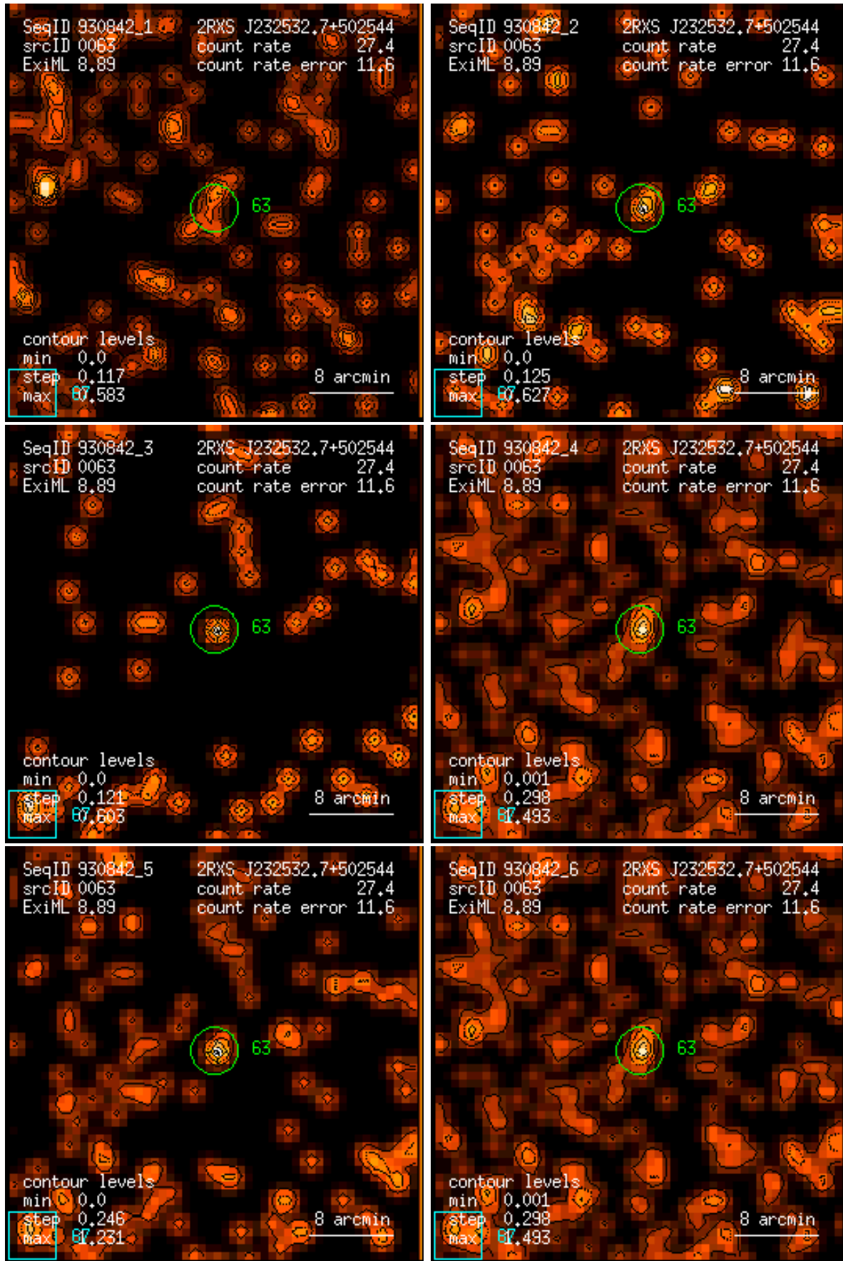
Figure 63: RASS 930842: detection 0063: band rate images, Gaussian filter: (1) PSPC channels 11 – 41, (2) 52 – 90, (3) 91 – 201, (4) 11 – 235, (5) 52 – 201, (6) 11 – 201. Broad band rates in counts/ks. Band rate contour levels in counts/ks/arcmin 2 .
