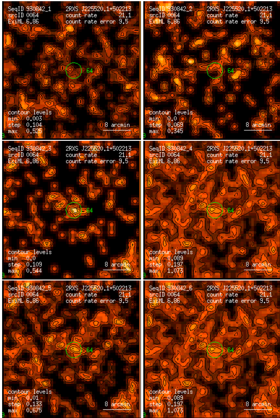
Figure 64: RASS 930842: detection 0064: band rate images, Gaussian filter: (1) PSPC channels 11 – 41, (2) 52 – 90, (3) 91 – 201, (4) 11 – 235, (5) 52 – 201, (6) 11 – 201. Broad band rates in counts/ks. Band rate contour levels in counts/ks/arcmin 2 .
