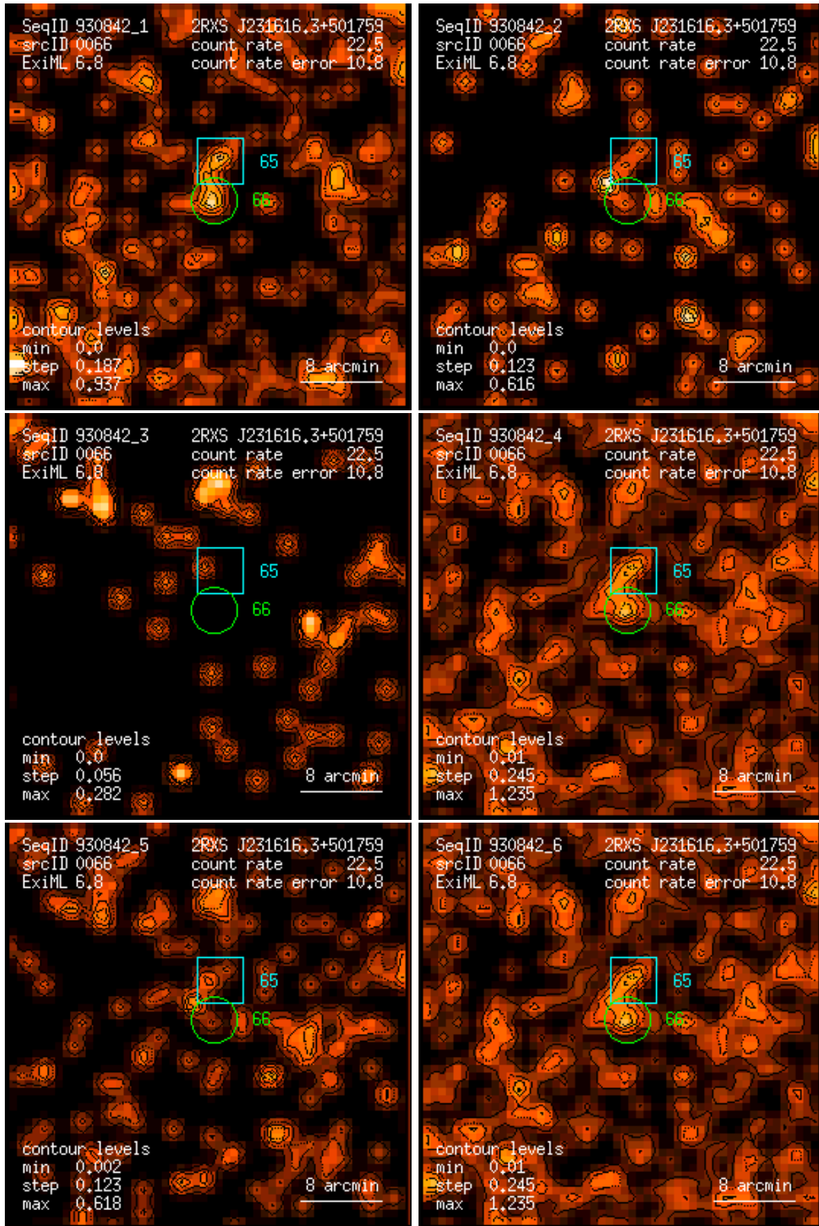
Figure 66: RASS 930842: detection 0066: band rate images, Gaussian filter: (1) PSPC channels 11 – 41, (2) 52 – 90, (3) 91 – 201, (4) 11 – 235, (5) 52 – 201, (6) 11 – 201. Broad band rates in counts/ks. Band rate contour levels in counts/ks/arcmin 2 .
