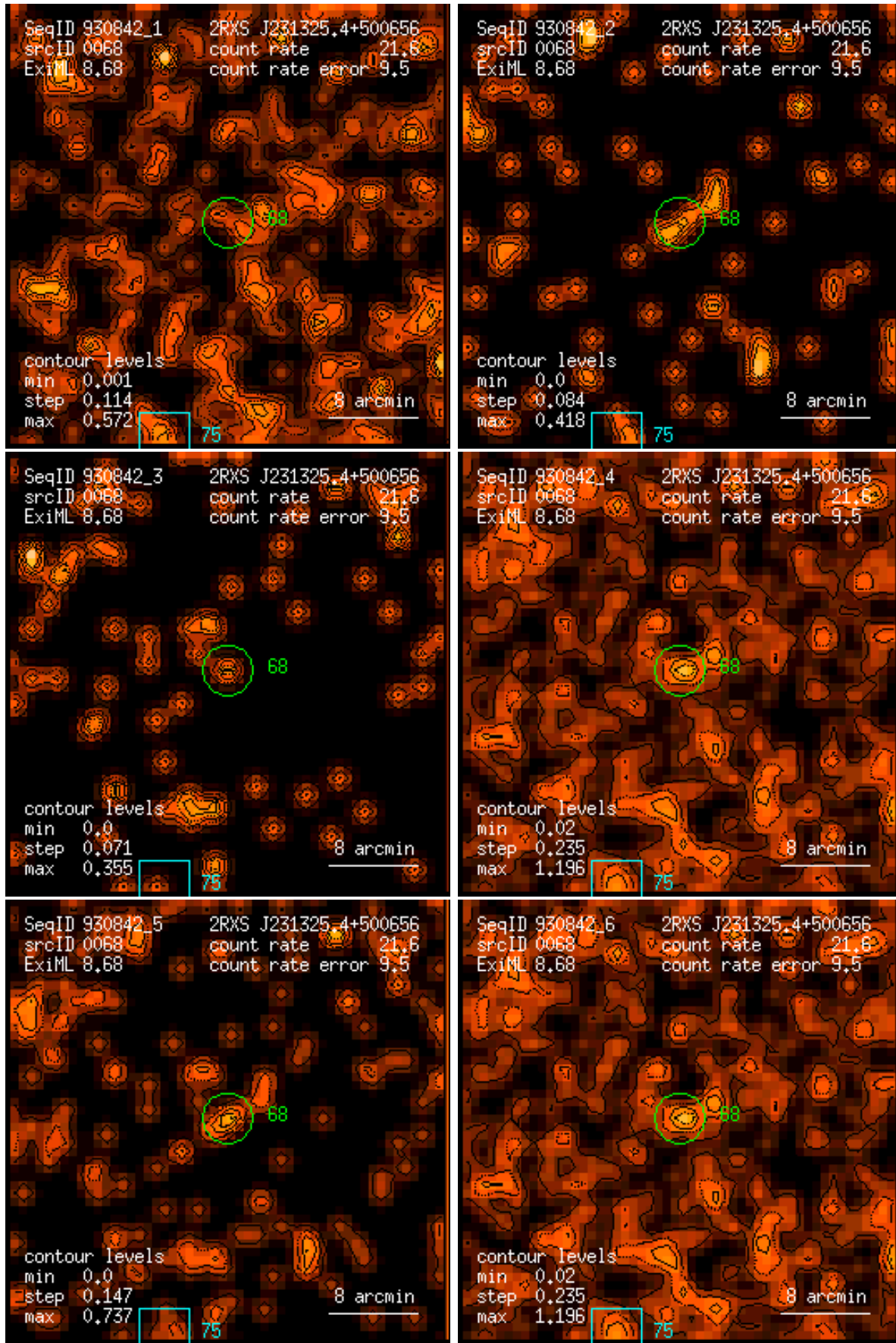
Figure 68: RASS 930842: detection 0068: band rate images, Gaussian filter: (1) PSPC channels 11 – 41, (2) 52 – 90, (3) 91 – 201, (4) 11 – 235, (5) 52 – 201, (6) 11 – 201. Broad band rates in counts/ks. Band rate contour levels in counts/ks/arcmin 2 .
