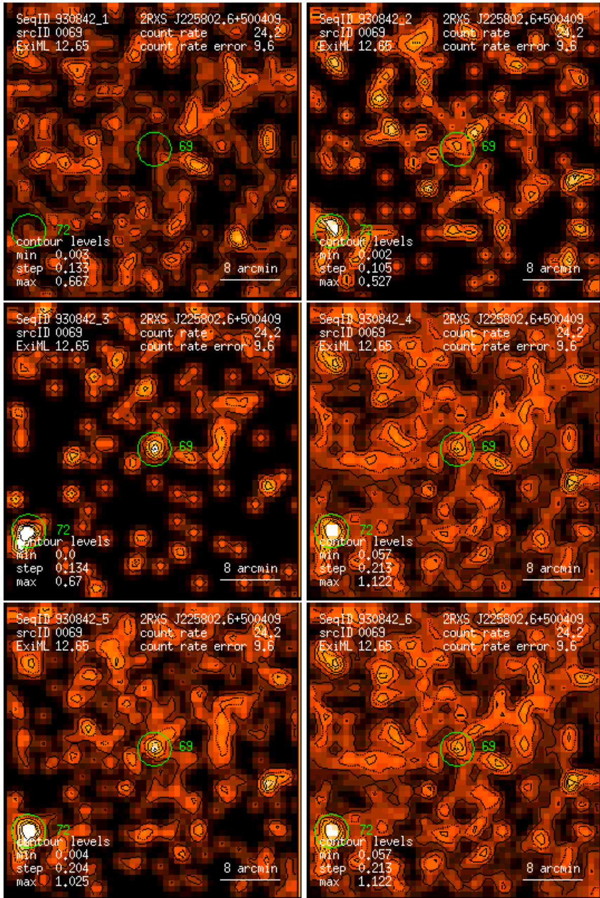
Figure 69: RASS 930842: detection 0069: band rate images, Gaussian filter: (1) PSPC channels 11 – 41, (2) 52 – 90, (3) 91 – 201, (4) 11 – 235, (5) 52 – 201, (6) 11 – 201. Broad band rates in counts/ks. Band rate contour levels in counts/ks/arcmin 2 .
