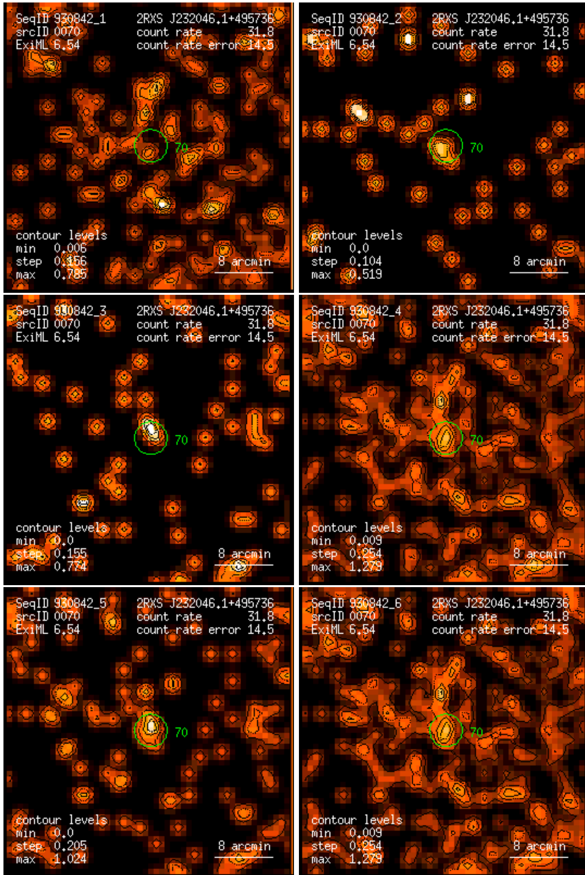
Figure 70: RASS 930842: detection 0070: band rate images, Gaussian filter: (1) PSPC channels 11 – 41, (2) 52 – 90, (3) 91 – 201, (4) 11 – 235, (5) 52 – 201, (6) 11 – 201. Broad band rates in counts/ks. Band rate contour levels in counts/ks/arcmin 2 .
