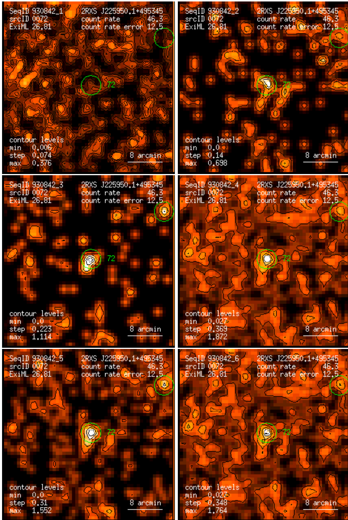
Figure 72: RASS 930842: detection 0072: band rate images, Gaussian filter: (1) PSPC channels 11 – 41, (2) 52 – 90, (3) 91 – 201, (4) 11 – 235, (5) 52 – 201, (6) 11 – 201. Broad band rates in counts/ks. Band rate contour levels in counts/ks/arcmin 2 .
