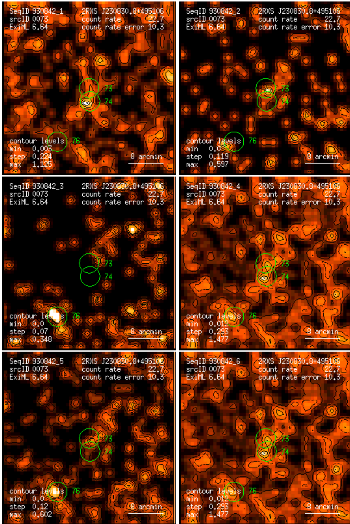
Figure 73: RASS 930842: detection 0073: band rate images, Gaussian filter: (1) PSPC channels 11 – 41, (2) 52 – 90, (3) 91 – 201, (4) 11 – 235, (5) 52 – 201, (6) 11 – 201. Broad band rates in counts/ks. Band rate contour levels in counts/ks/arcmin 2 .
