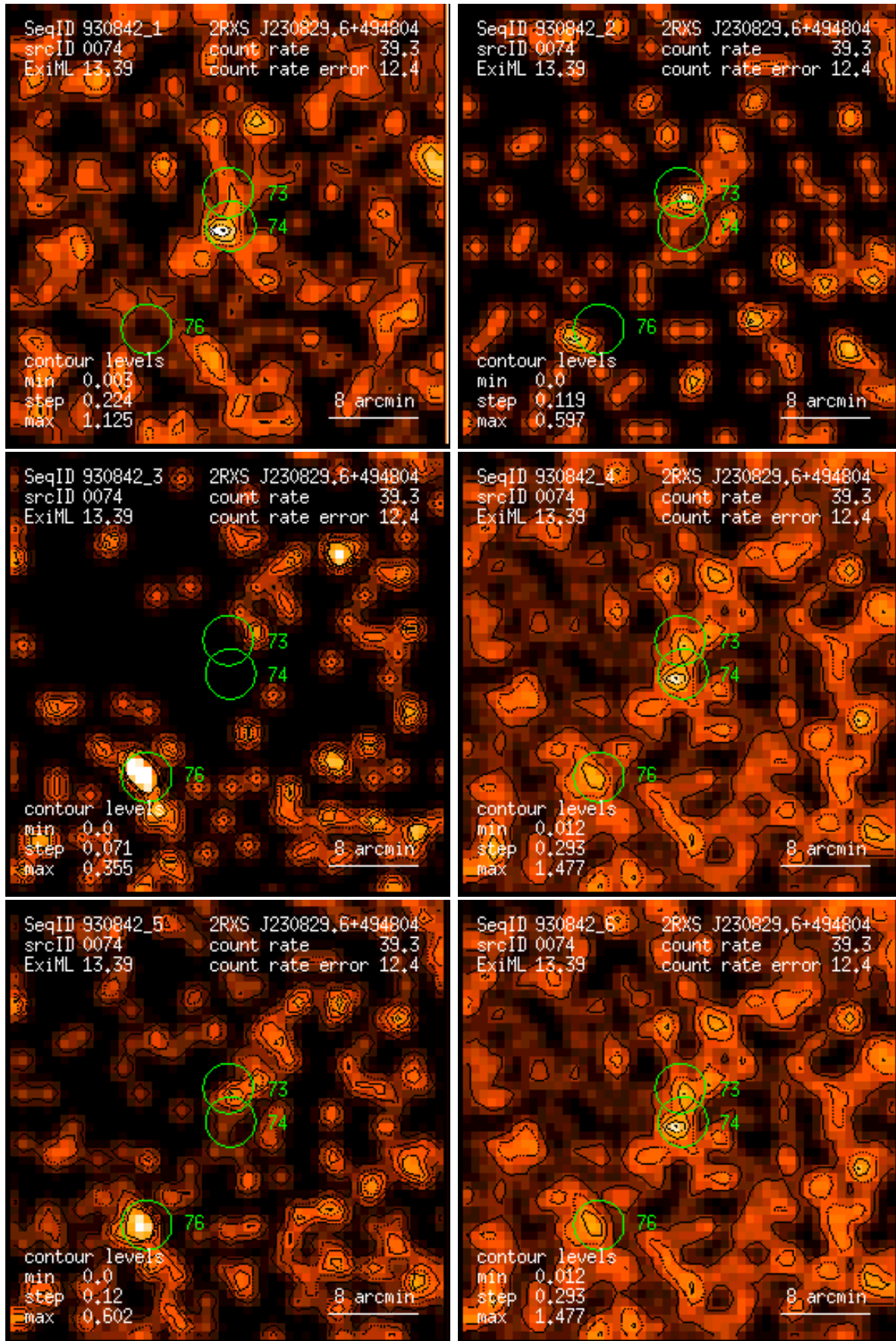
Figure 74: RASS 930842: detection 0074: band rate images, Gaussian filter: (1) PSPC channels 11 – 41, (2) 52 – 90, (3) 91 – 201, (4) 11 – 235, (5) 52 – 201, (6) 11 – 201. Broad band rates in counts/ks. Band rate contour levels in counts/ks/arcmin 2 .
