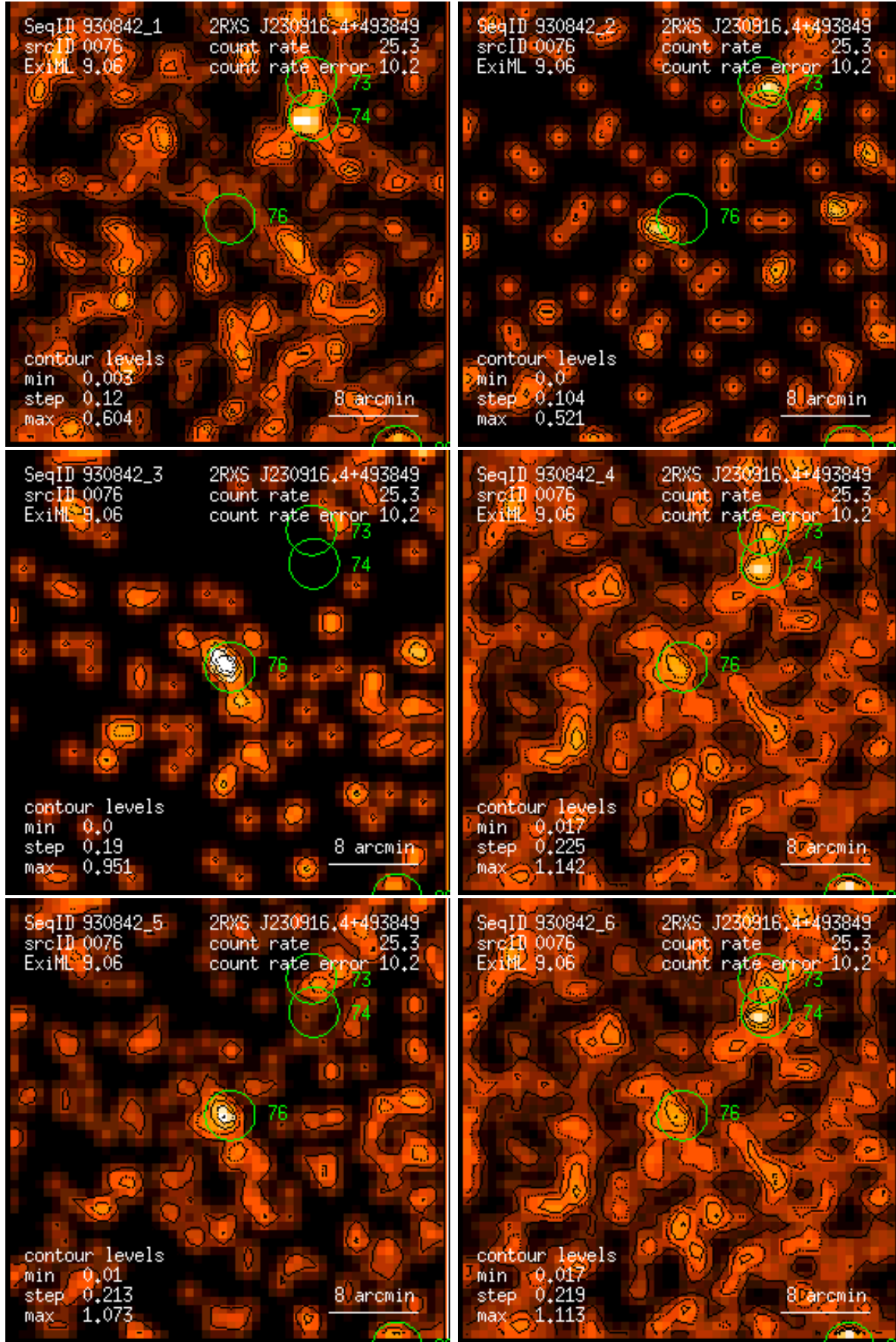
Figure 76: RASS 930842: detection 0076: band rate images, Gaussian filter: (1) PSPC channels 11 – 41, (2) 52 – 90, (3) 91 – 201, (4) 11 – 235, (5) 52 – 201, (6) 11 – 201. Broad band rates in counts/ks. Band rate contour levels in counts/ks/arcmin 2 .
