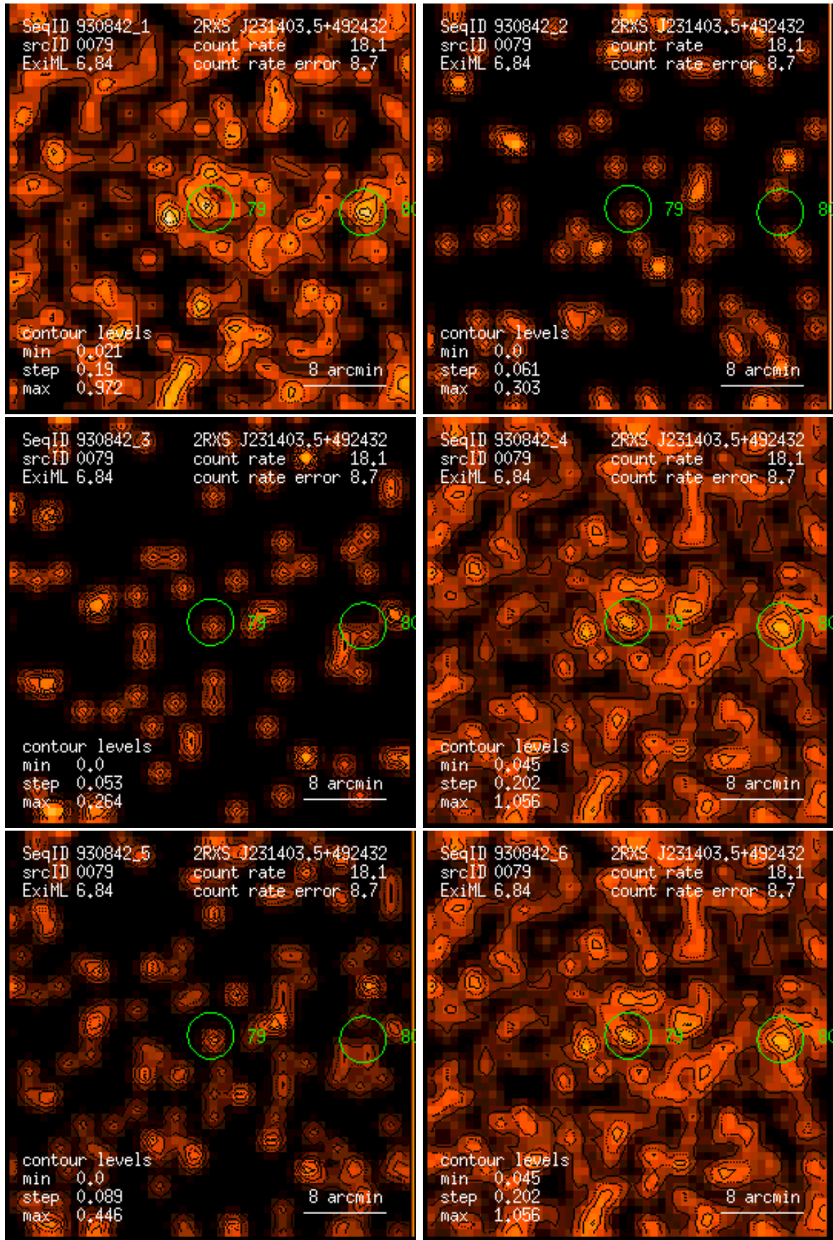
Figure 79: RASS 930842: detection 0079: band rate images, Gaussian filter: (1) PSPC channels 11 – 41, (2) 52 – 90, (3) 91 – 201, (4) 11 – 235, (5) 52 – 201, (6) 11 – 201. Broad band rates in counts/ks. Band rate contour levels in counts/ks/arcmin 2 .
