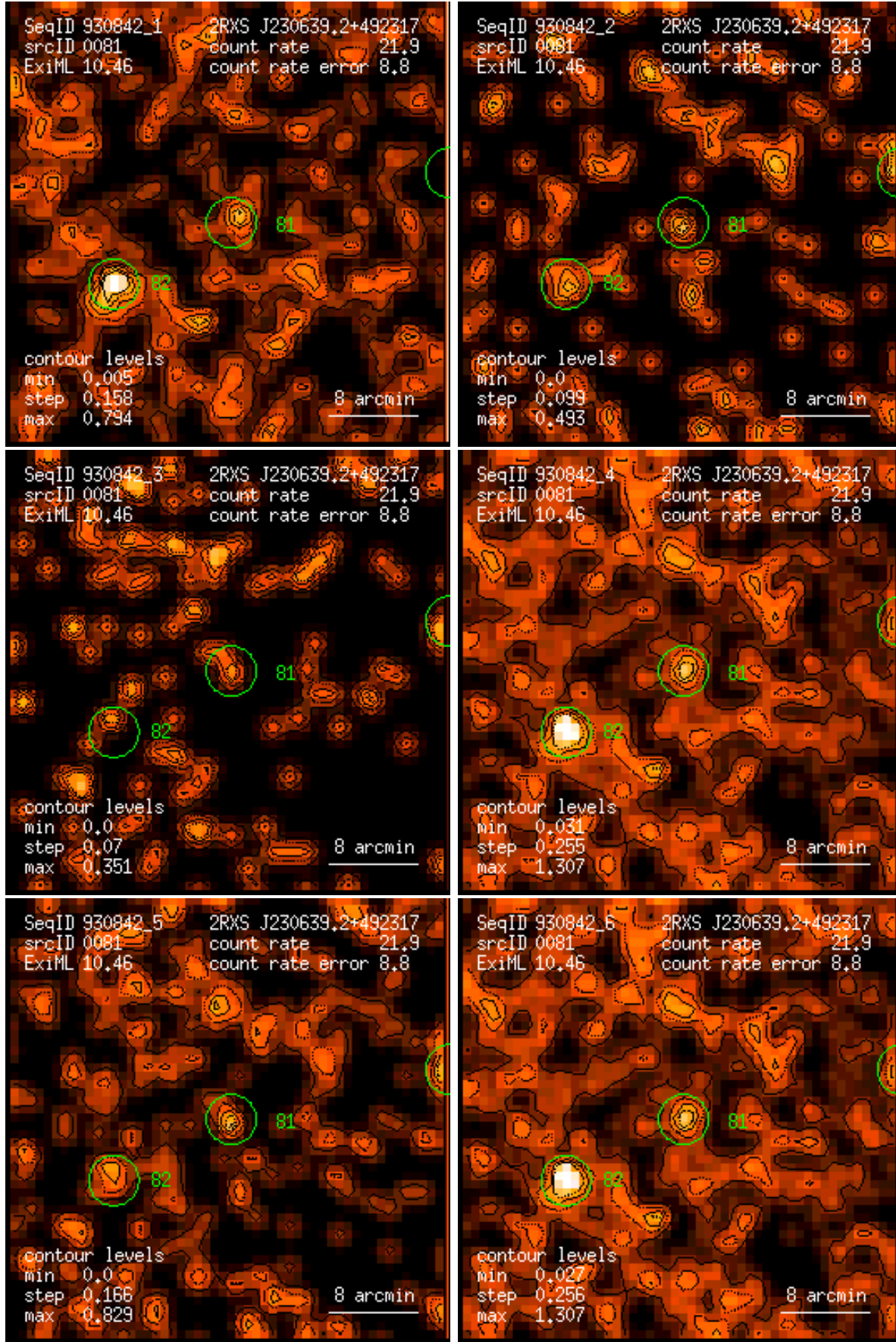
Figure 81: RASS 930842: detection 0081: band rate images, Gaussian filter: (1) PSPC channels 11 – 41, (2) 52 – 90, (3) 91 – 201, (4) 11 – 235, (5) 52 – 201, (6) 11 – 201. Broad band rates in counts/ks. Band rate contour levels in counts/ks/arcmin 2 .
