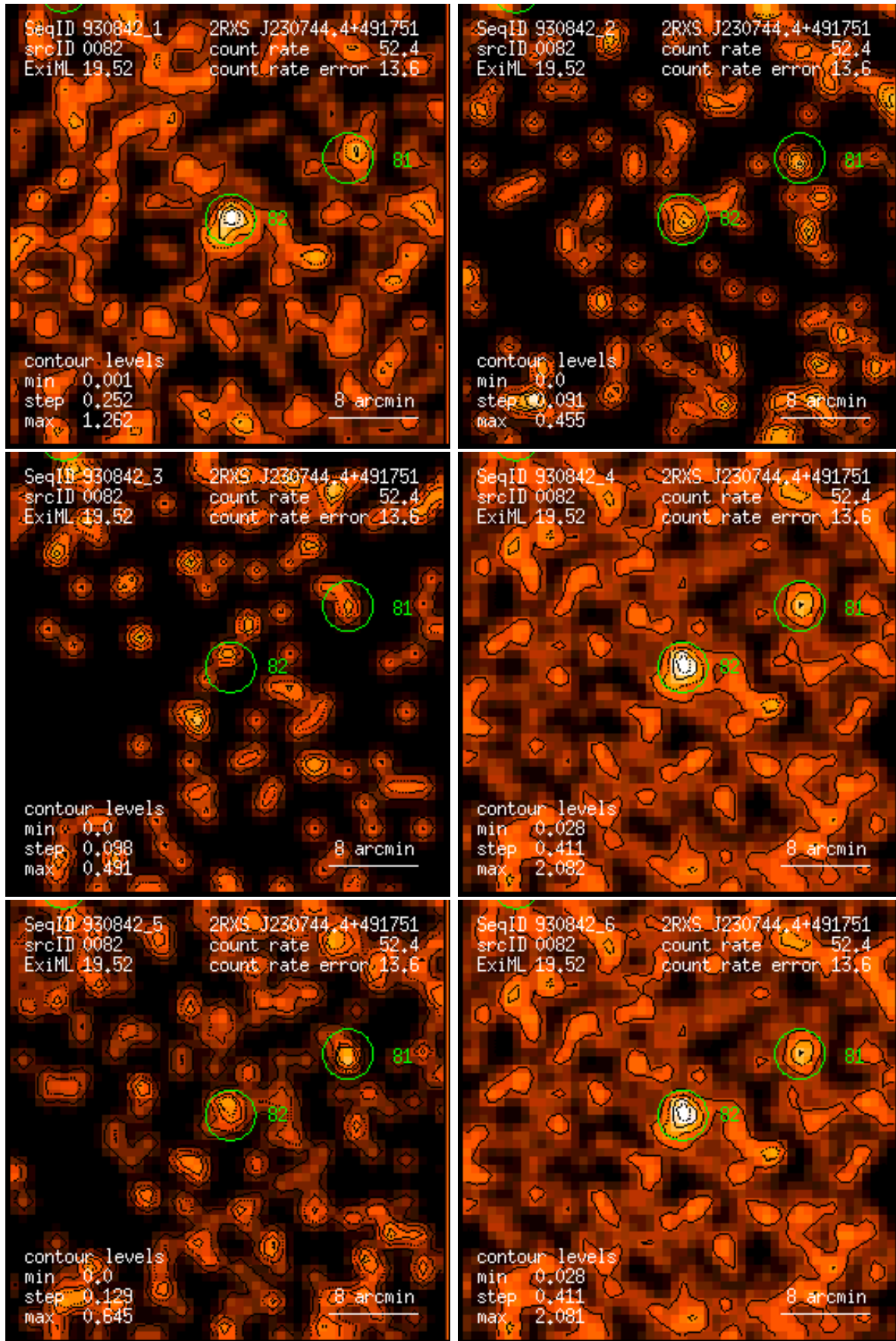
Figure 82: RASS 930842: detection 0082: band rate images, Gaussian filter: (1) PSPC channels 11 – 41, (2) 52 – 90, (3) 91 – 201, (4) 11 – 235, (5) 52 – 201, (6) 11 – 201. Broad band rates in counts/ks. Band rate contour levels in counts/ks/arcmin 2 .
