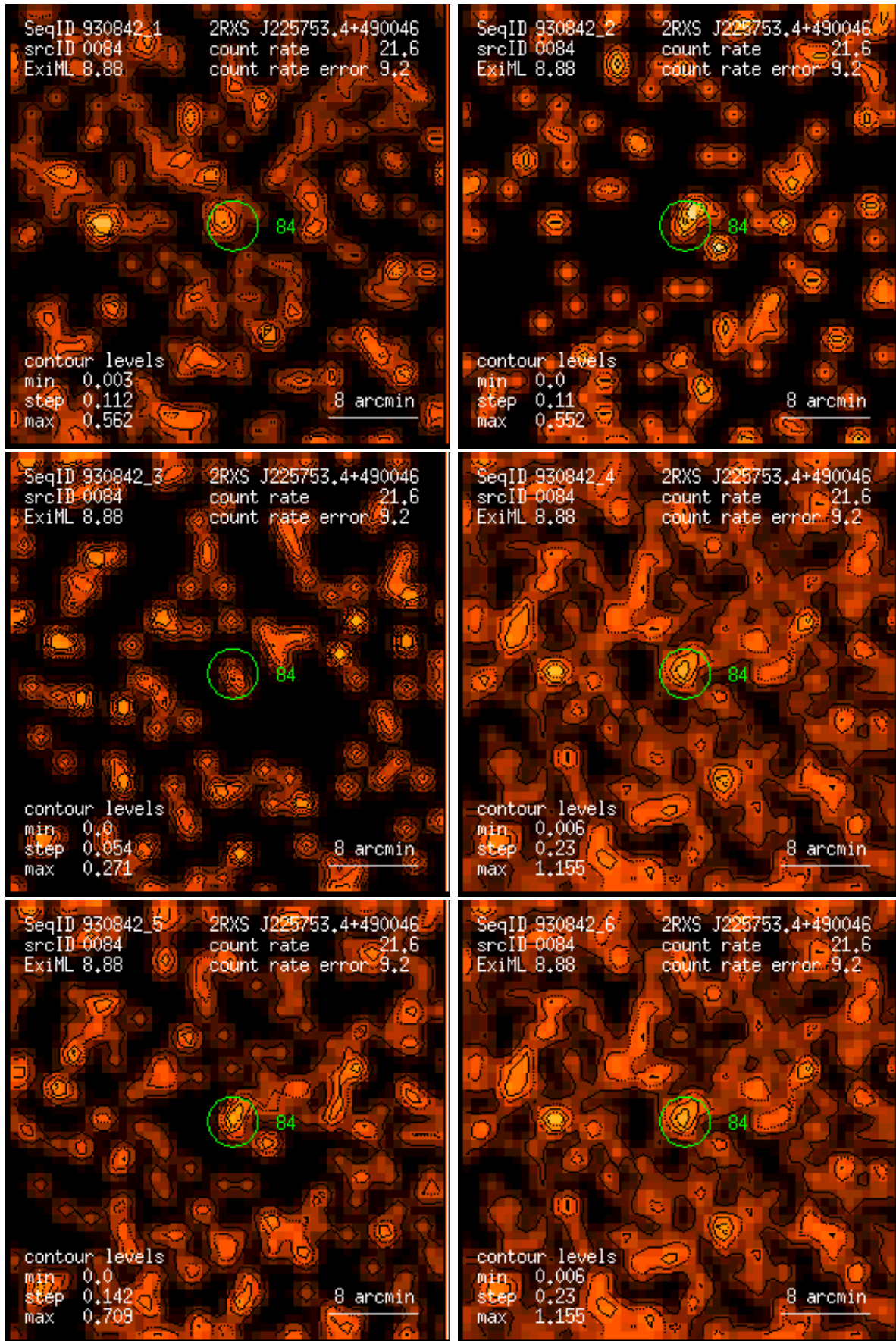
Figure 84: RASS 930842: detection 0084: band rate images, Gaussian filter: (1) PSPC channels 11 – 41, (2) 52 – 90, (3) 91 – 201, (4) 11 – 235, (5) 52 – 201, (6) 11 – 201. Broad band rates in counts/ks. Band rate contour levels in counts/ks/arcmin 2 .
