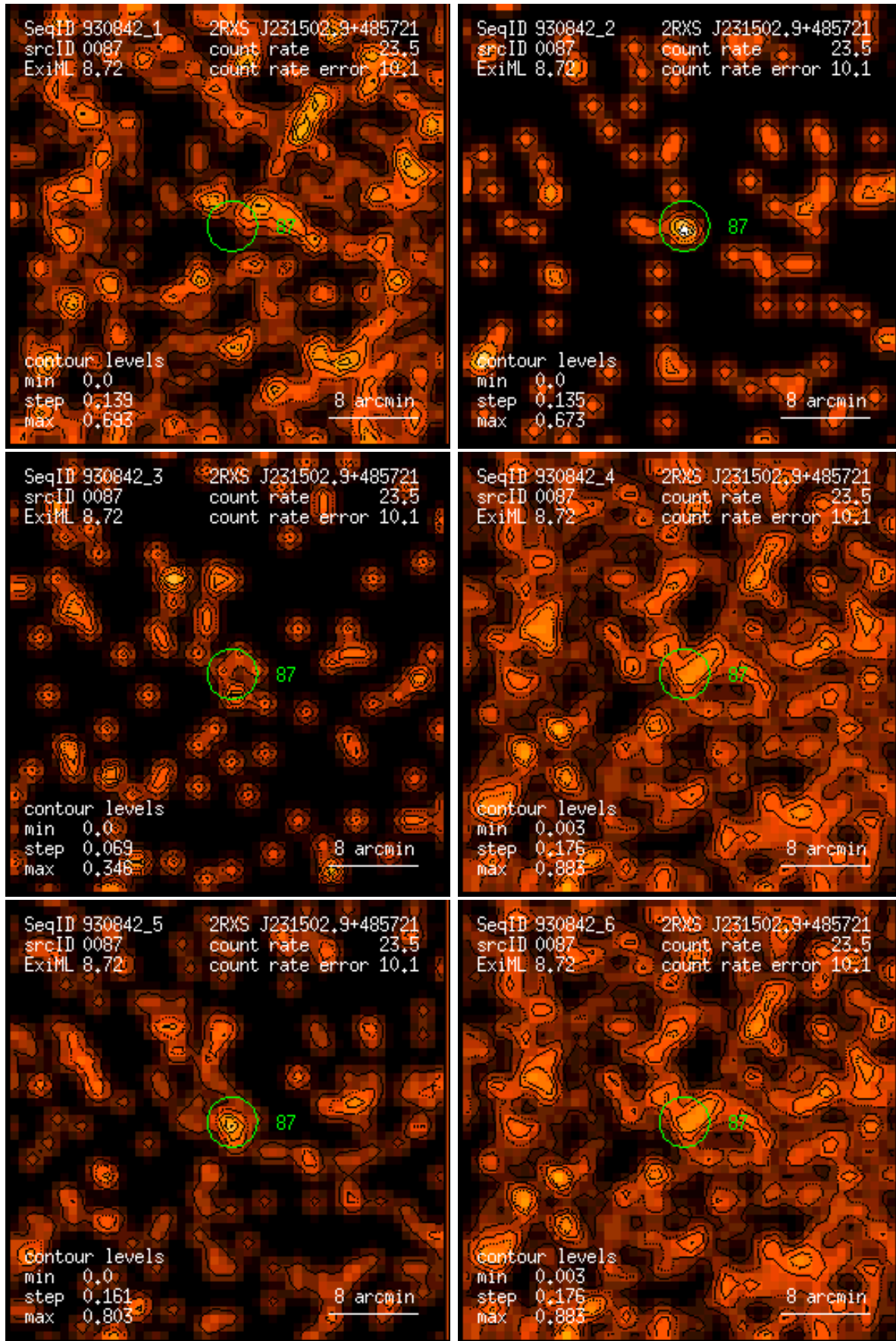
Figure 87: RASS 930842: detection 0087: band rate images, Gaussian filter: (1) PSPC channels 11 – 41, (2) 52 – 90, (3) 91 – 201, (4) 11 – 235, (5) 52 – 201, (6) 11 – 201. Broad band rates in counts/ks. Band rate contour levels in counts/ks/arcmin 2 .
