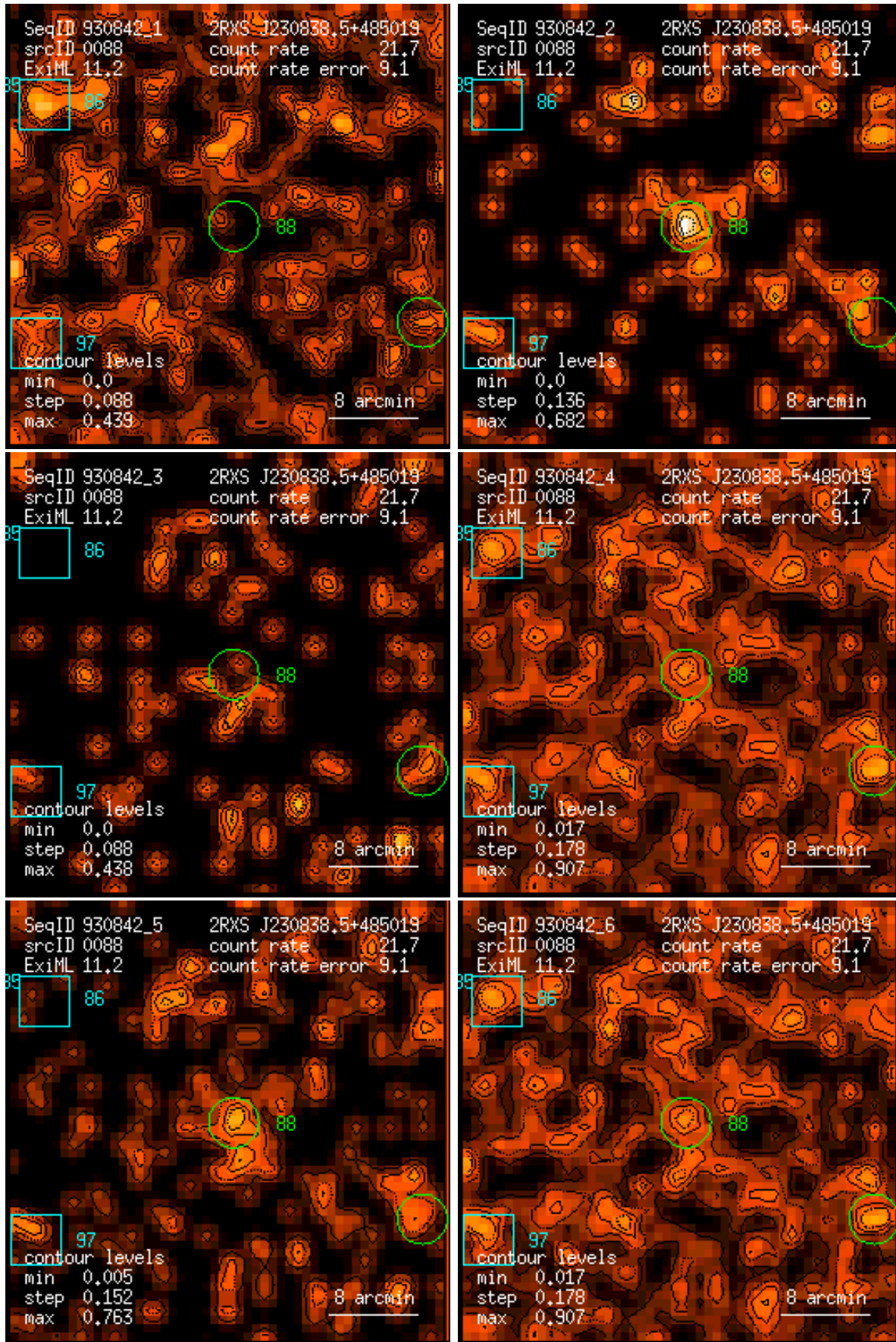
Figure 88: RASS 930842: detection 0088: band rate images, Gaussian filter: (1) PSPC channels 11 – 41, (2) 52 – 90, (3) 91 – 201, (4) 11 – 235, (5) 52 – 201, (6) 11 – 201. Broad band rates in counts/ks. Band rate contour levels in counts/ks/arcmin 2 .
