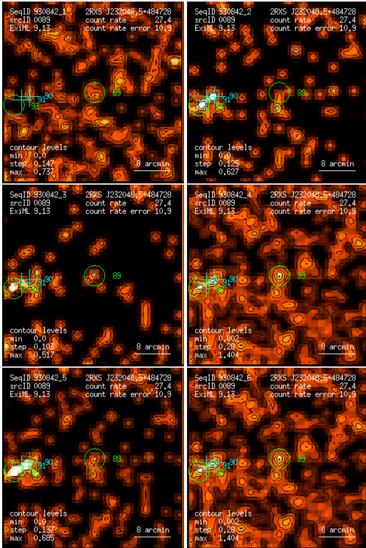
Figure 89: RASS 930842: detection 0089: band rate images, Gaussian filter: (1) PSPC channels 11 – 41, (2) 52 – 90, (3) 91 – 201, (4) 11 – 235, (5) 52 – 201, (6) 11 – 201. Broad band rates in counts/ks. Band rate contour levels in counts/ks/arcmin 2 .
