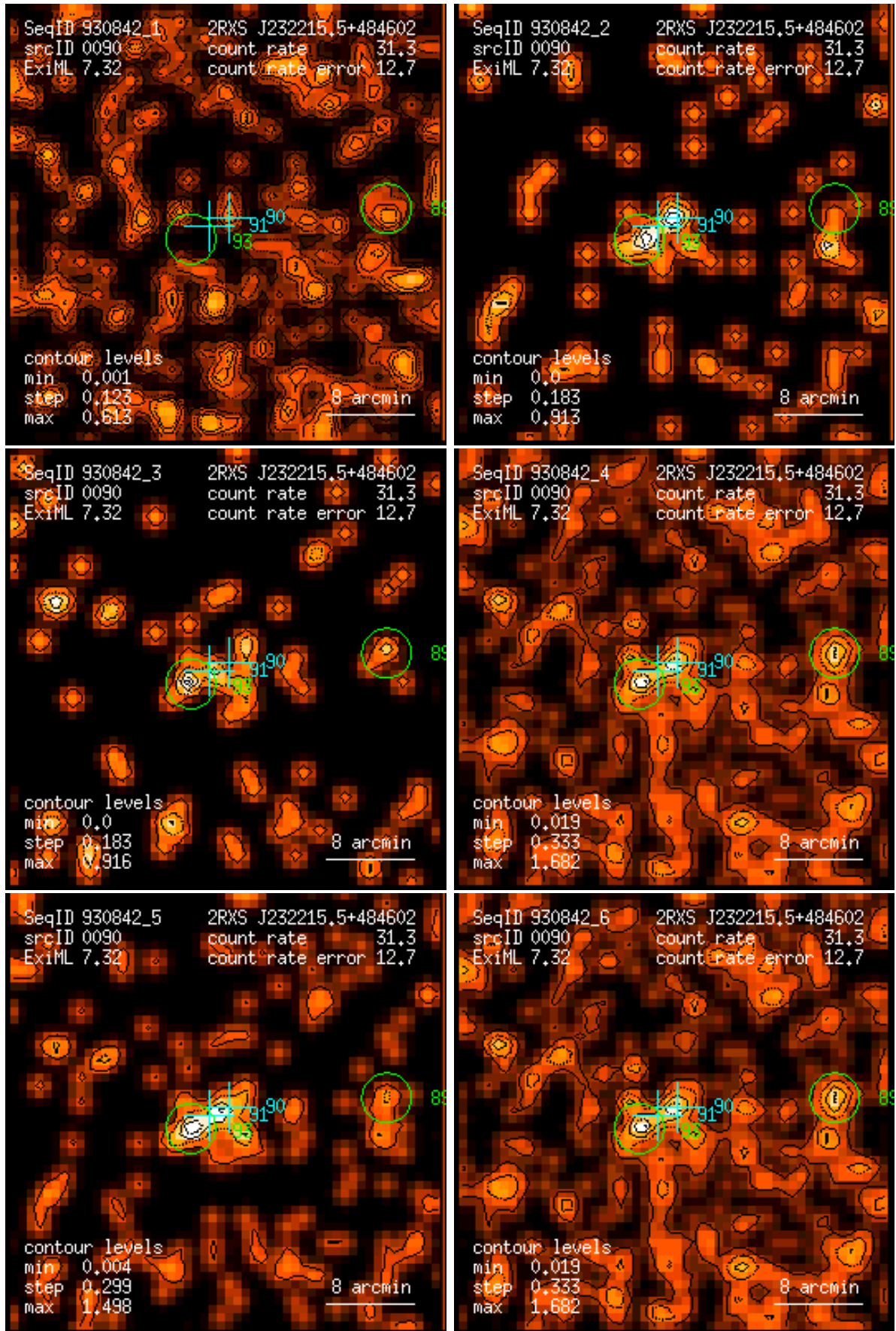
Figure 90: RASS 930842: detection 0090: band rate images, Gaussian filter: (1) PSPC channels 11 – 41, (2) 52 – 90, (3) 91 – 201, (4) 11 – 235, (5) 52 – 201, (6) 11 – 201. Broad band rates in counts/ks. Band rate contour levels in counts/ks/arcmin 2 .
