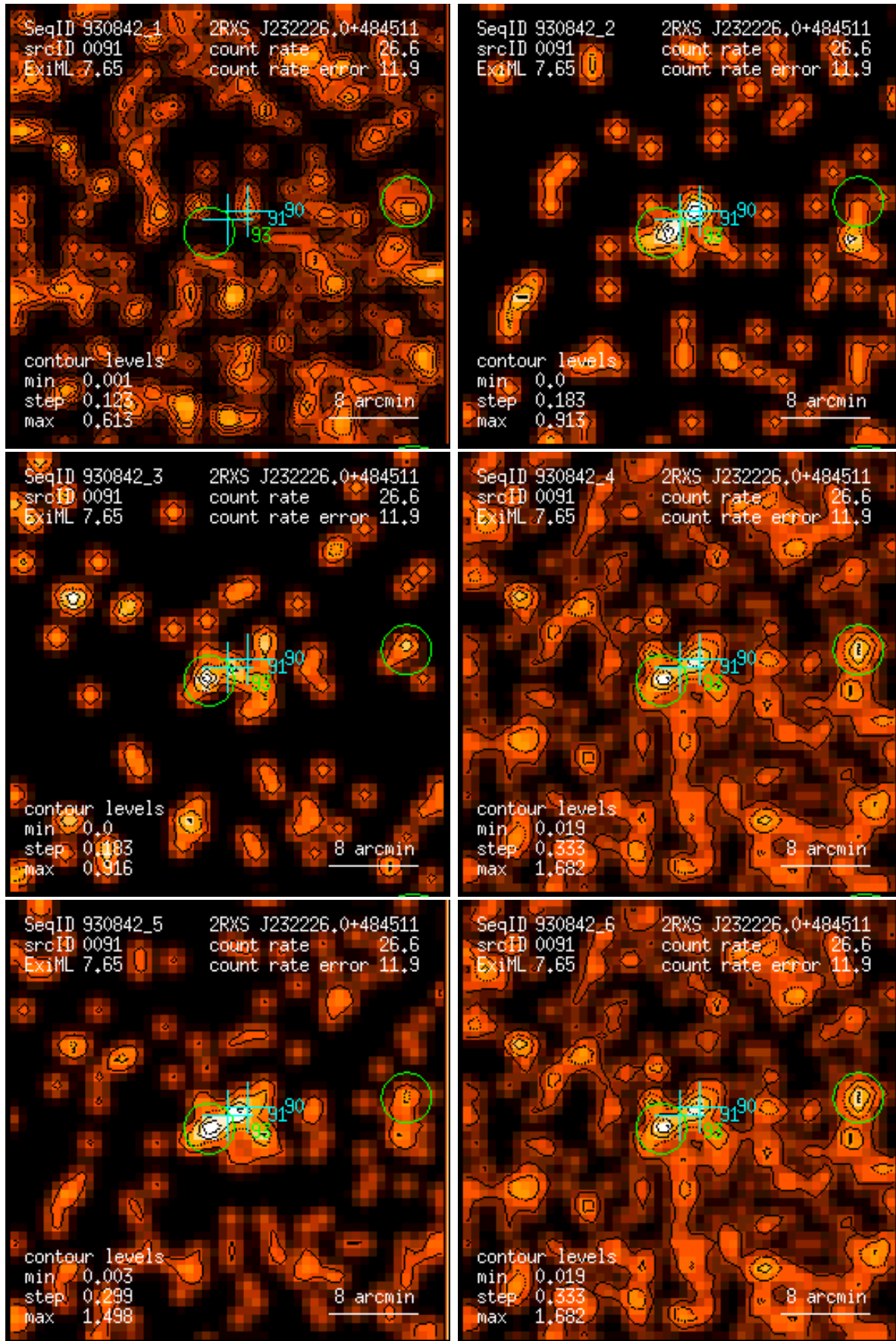
Figure 91: RASS 930842: detection 0091: band rate images, Gaussian filter: (1) PSPC channels 11 – 41, (2) 52 – 90, (3) 91 – 201, (4) 11 – 235, (5) 52 – 201, (6) 11 – 201. Broad band rates in counts/ks. Band rate contour levels in counts/ks/arcmin 2 .
