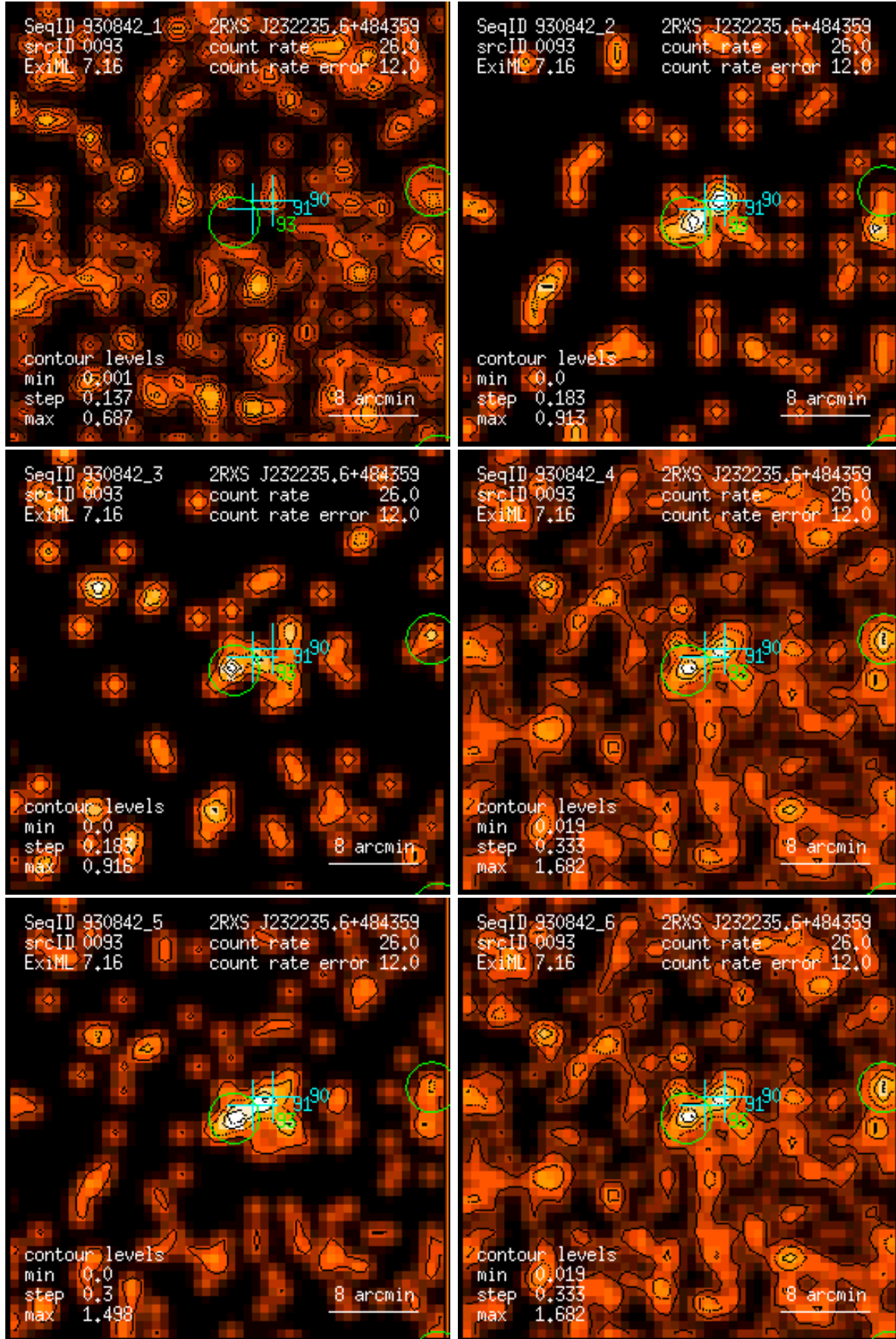
Figure 93: RASS 930842: detection 0093: band rate images, Gaussian filter: (1) PSPC channels 11 – 41, (2) 52 – 90, (3) 91 – 201, (4) 11 – 235, (5) 52 – 201, (6) 11 – 201. Broad band rates in counts/ks. Band rate contour levels in counts/ks/arcmin 2 .
