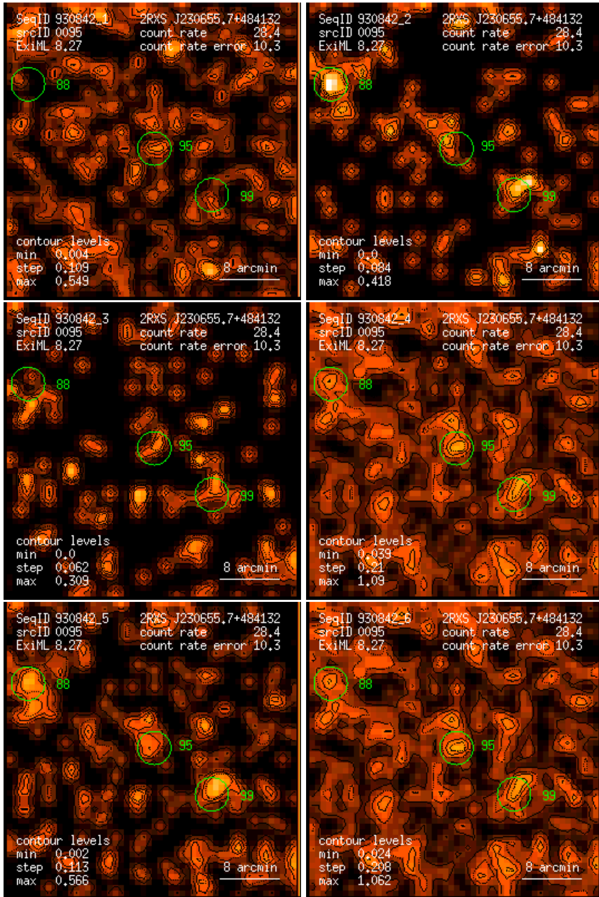
Figure 95: RASS 930842: detection 0095: band rate images, Gaussian filter: (1) PSPC channels 11 – 41, (2) 52 – 90, (3) 91 – 201, (4) 11 – 235, (5) 52 – 201, (6) 11 – 201. Broad band rates in counts/ks. Band rate contour levels in counts/ks/arcmin 2 .
