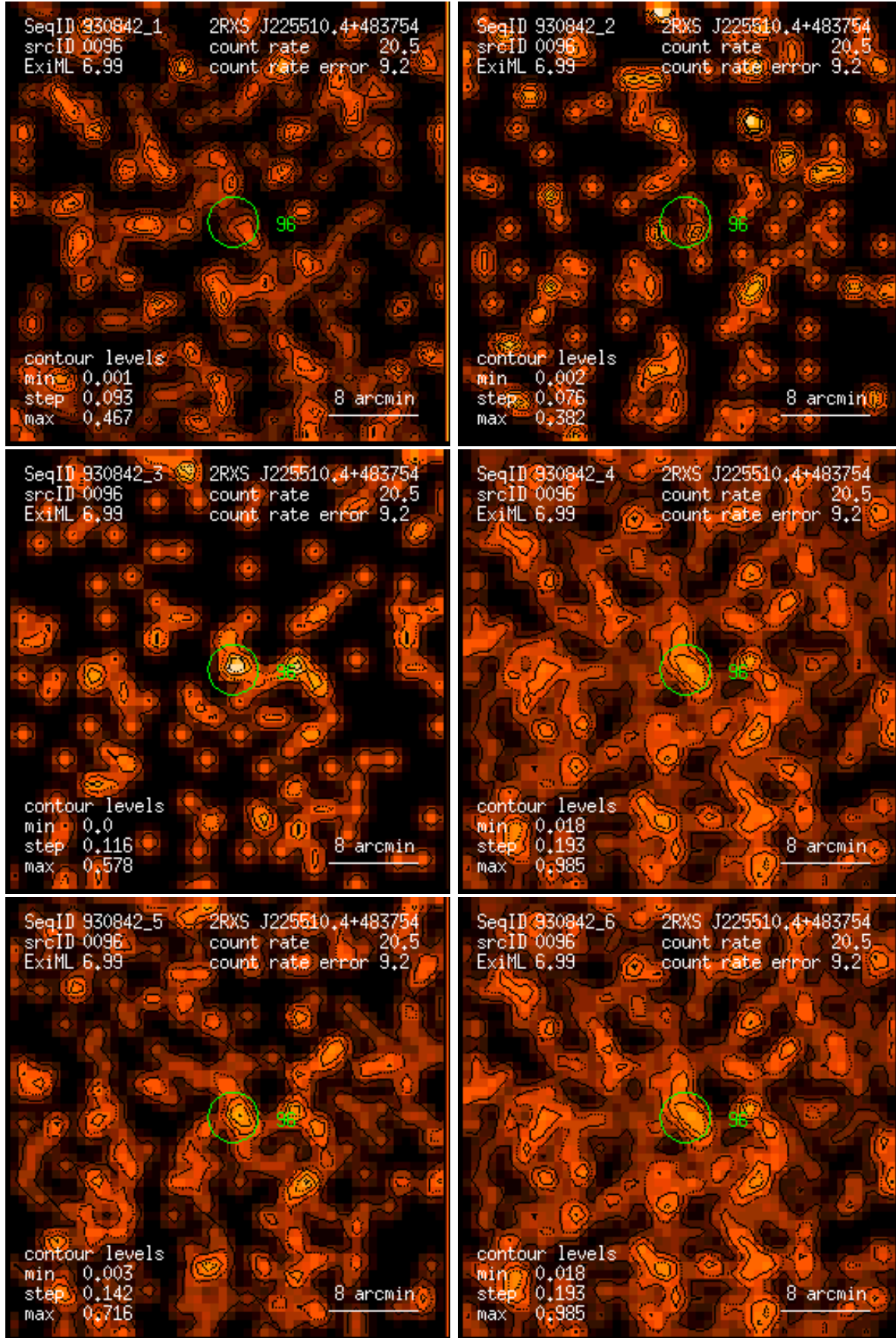
Figure 96: RASS 930842: detection 0096: band rate images, Gaussian filter: (1) PSPC channels 11 – 41, (2) 52 – 90, (3) 91 – 201, (4) 11 – 235, (5) 52 – 201, (6) 11 – 201. Broad band rates in counts/ks. Band rate contour levels in counts/ks/arcmin 2 .
