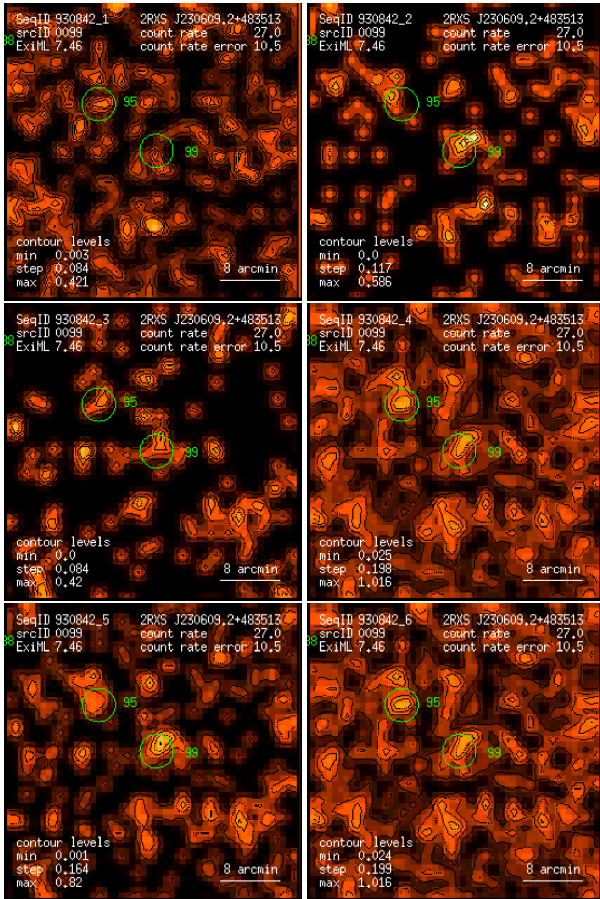
Figure 99: RASS 930842: detection 0099: band rate images, Gaussian filter: (1) PSPC channels 11 – 41, (2) 52 – 90, (3) 91 – 201, (4) 11 – 235, (5) 52 – 201, (6) 11 – 201. Broad band rates in counts/ks. Band rate contour levels in counts/ks/arcmin 2 .
