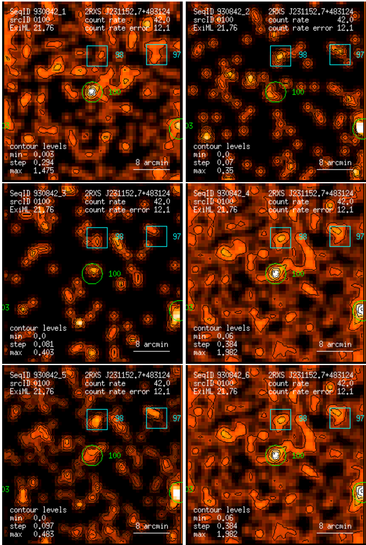
Figure 100: RASS 930842: detection 0100: band rate images, Gaussian filter: (1) PSPC channels 11 – 41, (2) 52 – 90, (3) 91 – 201, (4) 11 – 235, (5) 52 – 201, (6) 11 – 201. Broad band rates in counts/ks. Band rate contour levels in counts/ks/arcmin 2 .
