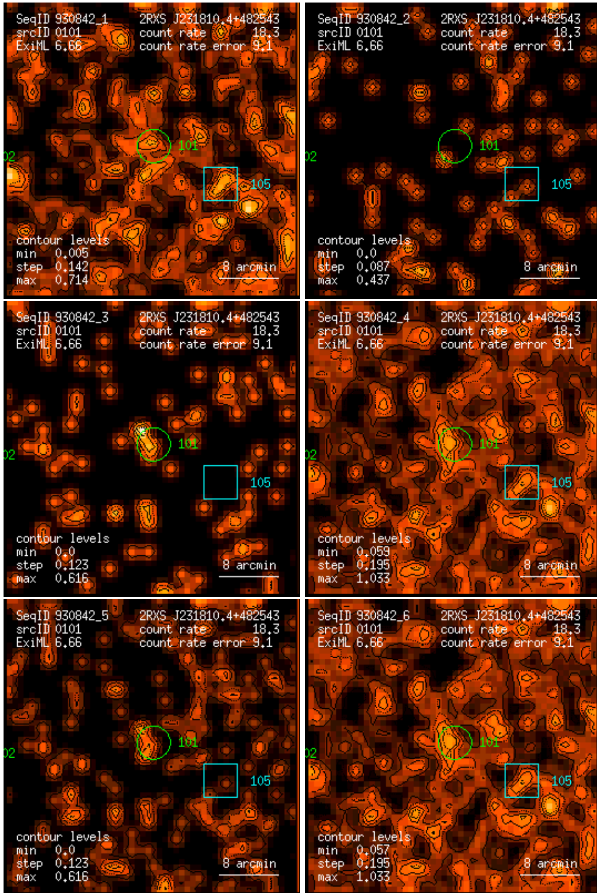
Figure 101: RASS 930842: detection 0101: band rate images, Gaussian filter: (1) PSPC channels 11 – 41, (2) 52 – 90, (3) 91 – 201, (4) 11 – 235, (5) 52 – 201, (6) 11 – 201. Broad band rates in counts/ks. Band rate contour levels in counts/ks/arcmin 2 .
