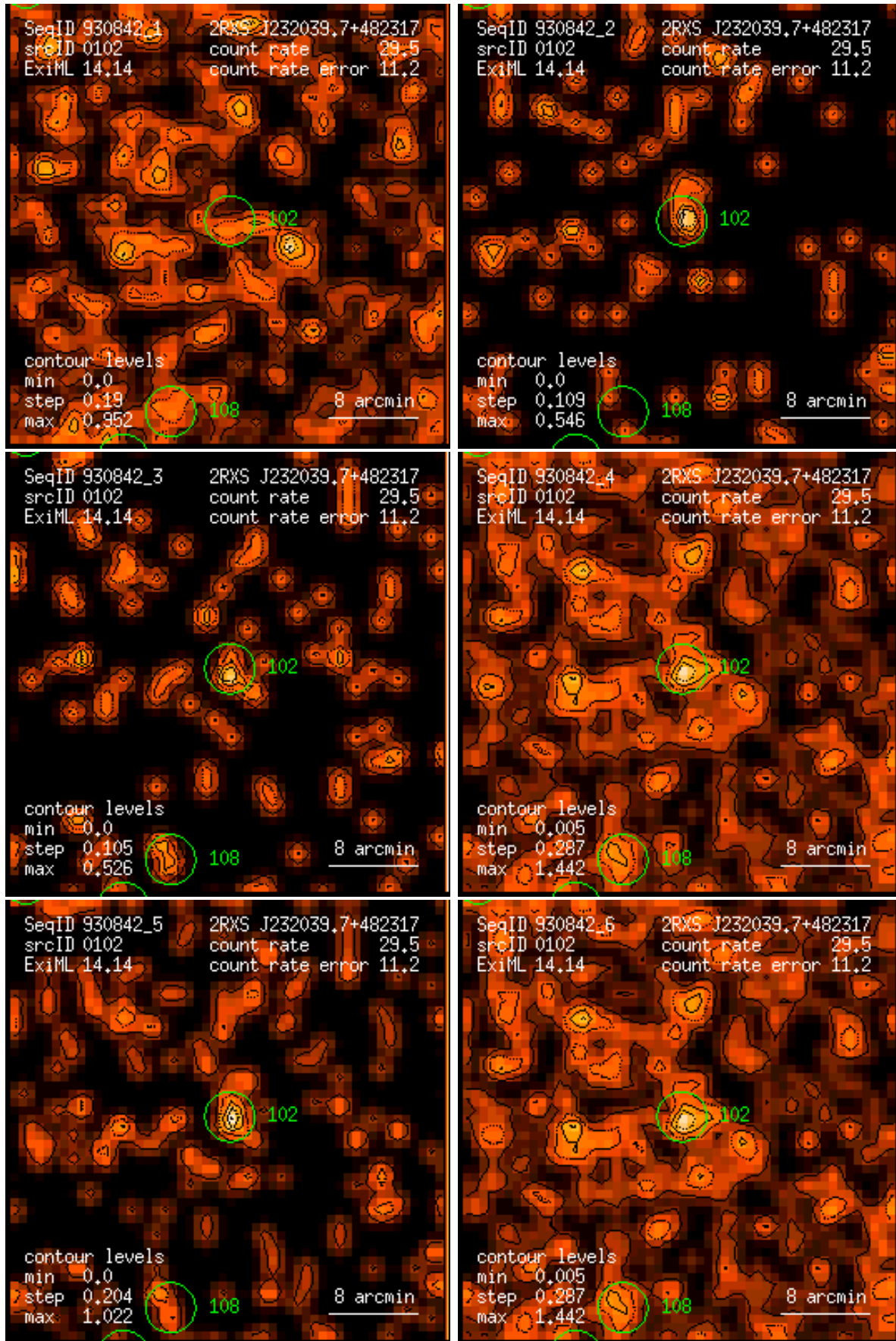
Figure 102: RASS 930842: detection 0102: band rate images, Gaussian filter: (1) PSPC channels 11 – 41, (2) 52 – 90, (3) 91 – 201, (4) 11 – 235, (5) 52 – 201, (6) 11 – 201. Broad band rates in counts/ks. Band rate contour levels in counts/ks/arcmin 2 .
