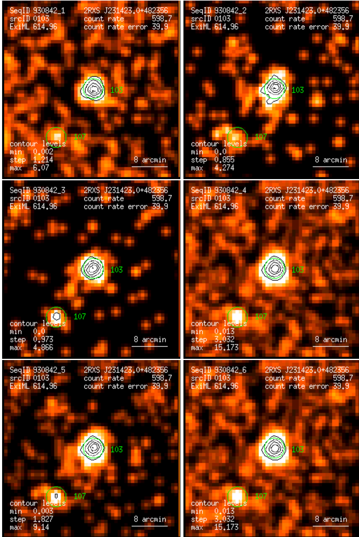
Figure 103: RASS 930842: detection 0103: band rate images, Gaussian filter: (1) PSPC channels 11 – 41, (2) 52 – 90, (3) 91 – 201, (4) 11 – 235, (5) 52 – 201, (6) 11 – 201. Broad band rates in counts/ks. Band rate contour levels in counts/ks/arcmin 2 .
