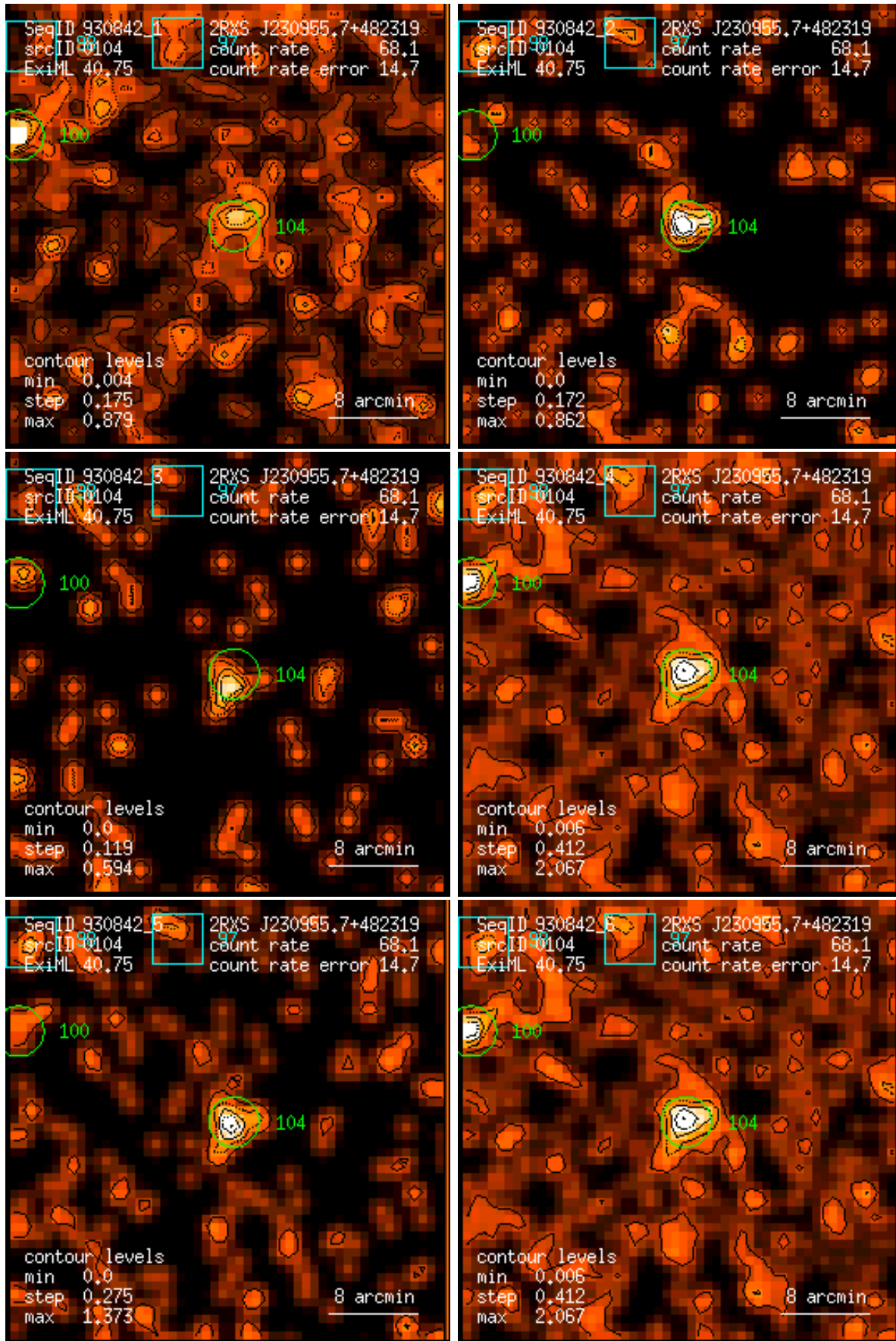
Figure 104: RASS 930842: detection 0104: band rate images, Gaussian filter: (1) PSPC channels 11 – 41, (2) 52 – 90, (3) 91 – 201, (4) 11 – 235, (5) 52 – 201, (6) 11 – 201. Broad band rates in counts/ks. Band rate contour levels in counts/ks/arcmin 2 .
