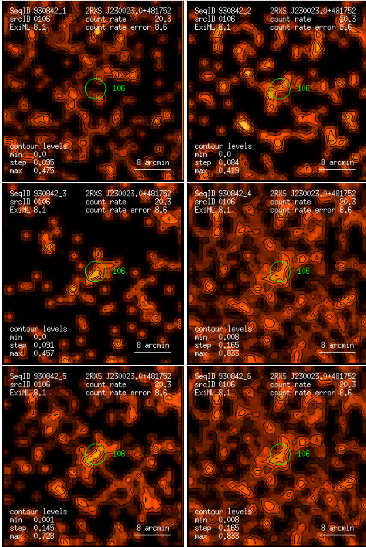
Figure 106: RASS 930842: detection 0106: band rate images, Gaussian filter: (1) PSPC channels 11 – 41, (2) 52 – 90, (3) 91 – 201, (4) 11 – 235, (5) 52 – 201, (6) 11 – 201. Broad band rates in counts/ks. Band rate contour levels in counts/ks/arcmin 2 .
